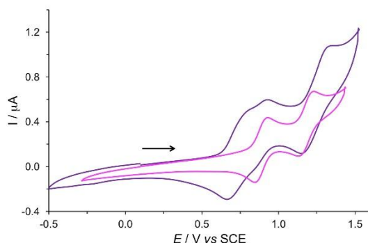
Figure 7. Cyclic voltammograms of compounds 16 (pink) and 20 (purple) on a Pt electrode in CH 2 Cl 2 + 0.1 M [ n Bu 4 N][BF 4 ] at a scan rate of 200 mV s -1 (toward anodic potentials).
