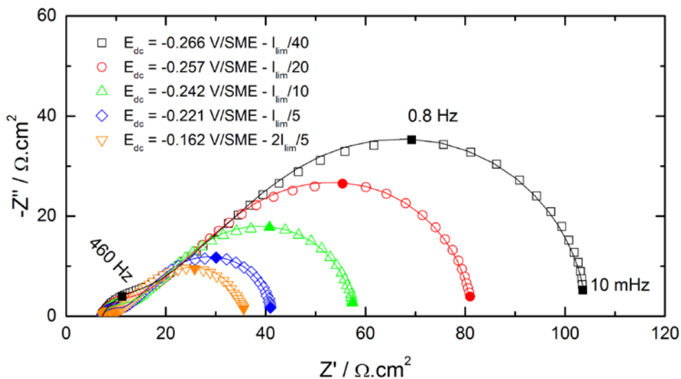
Figure 9: Nyquist plot of the impedance response for the ferrocyanide oxidation in 0.1 M K 2 SO 4 at a gold RDE as a function of the potential at 900 rpm – Symbols: experimental results; Solid line: fit with the equivalent circuit presented in Figure 5.
