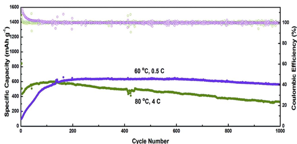
Figure 8. Discharge capacity (solid circle) and coulombic efficiencies (open circle) at 80 °C, 4C (dark yellow, after a three-cycle activation at 80 °C, 0.2C) and at 60 °C, 0.5C (purple), for a battery in which the cathode was fabricated from a slurry of PANI@C/S, carbon black (SuperP) and a binder (80:10:10 by weight). The electrolyte was a PEO–MIL-53(AI)–LiTFSI 60 \mu\text{m} -thick film [341]. Reproduced with permission from the Royal Society of Chemistry.
