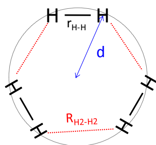
Figure 1. "3 H 2 " molecules confined in a ring and constrained to D_{3h} symmetry, the distance d being adjusted to model the effect of pressure.
