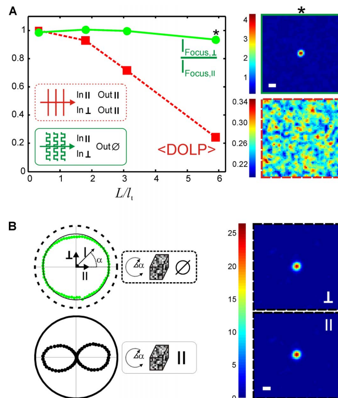
Fig. 2. Experimental quantification of polarization recovery. (A) Left: Averaged DOLP of the speckle (<DOLP>) (red squares) and refocus intensity ratio after wavefront shaping ( l_t/l_t ; corresponding to the same wavefront but rotated input polarization) (green circles), as a function of optical depths L/l_t . Polarization scrambling of the speckle occurs for lengths of l_t . Nevertheless, at depths of several l_t , after shaping, the refocus intensity survives a change of 90^\circ of the input polarization. Right: Speckle image after (top) and before (bottom) the wavefront shaping procedure. The scattering media are made of 5\text{-}\mu\text{m} -diameter polystyrene beads. The asterisk symbol (*) in the box refers to the images shown on the right. (B) Similar experiments performed using 1-mm-thick opaque acute brain slice coronal cross section as a scattering medium. Top left: Nonanalyzed refocus intensity (green circles) upon rotation of the excitation field. Right: Images show the refocus at two input polarization states ( \perp and \parallel ) with the same intensity scale. Bottom left: The refocus polarization state purity is evaluated by placing an analyzer and observing an extinction (black circles). Scale bars, 1\ \mu\text{m} .
