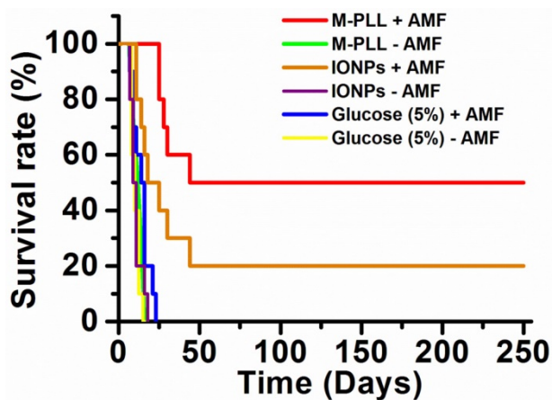
Figure 6. Survival rate of mice belonging to group 1 (M-PLL+AMF), group 2 (M-PLL-AMF), group 3 (IONPs+AMF), group 4 (IONPs-AMF), group 5 (Glucose (5%)+AMF), and group 6 (Glucose (5%)-AMF).
