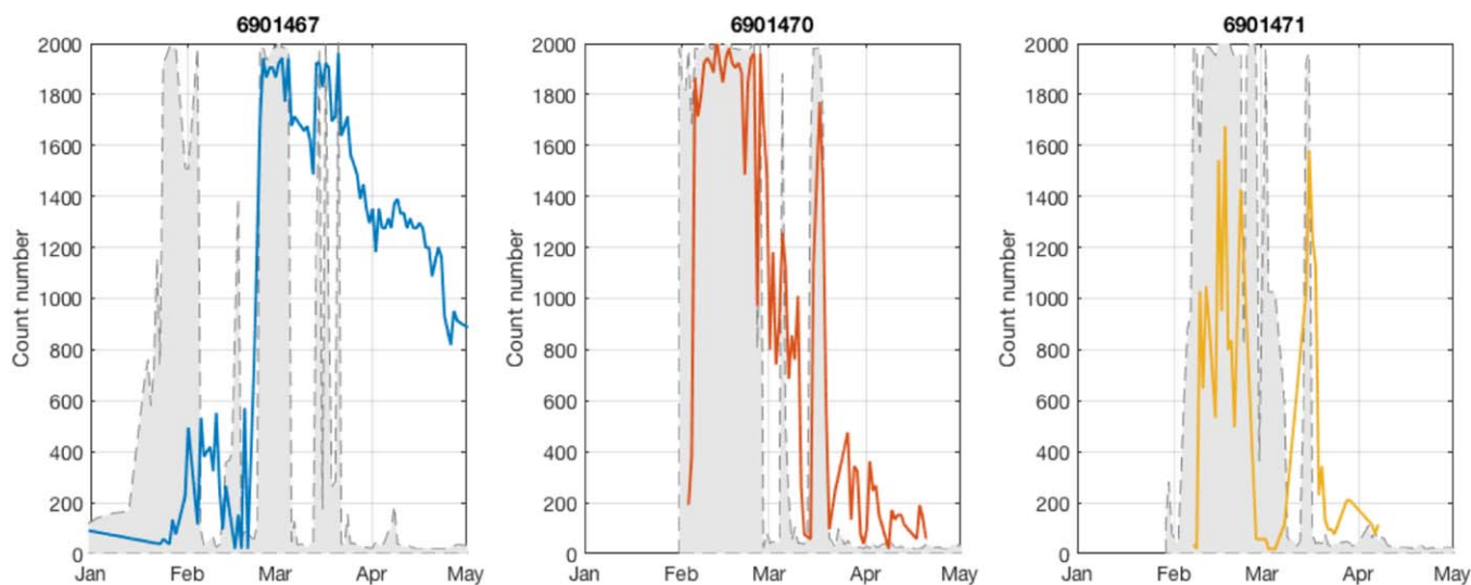
Figure 7. Evolution of count number of samples after interpolation for each meter of individual profile following the AOU and density thresholds ( <48 \mu\text{mol kg}^{-1} and >29.11 \text{ kg m}^{-3} ) for Argo floats 6901467 (blue), 6901470 (red), and 6901471 (yellow). The grey area in the background represents the ML depth observed by respective floats.
