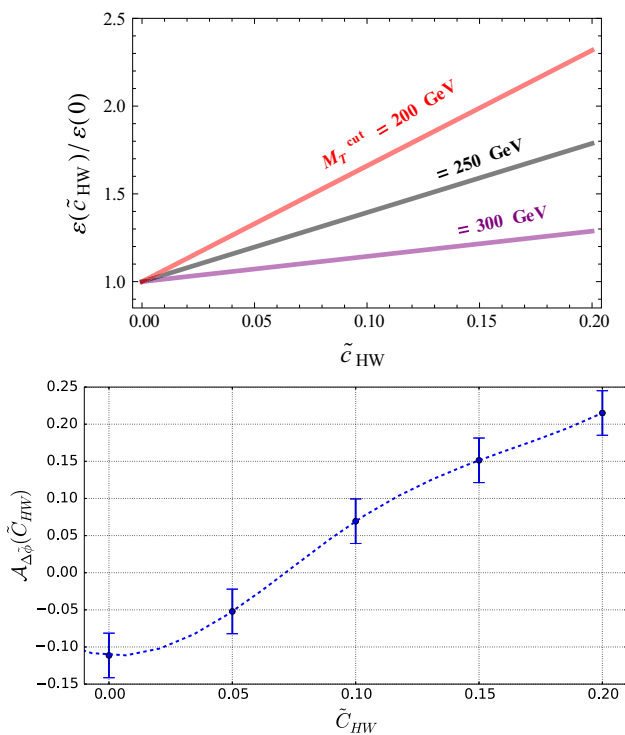
Fig. 8 Same as in Fig. 6 but for WH production
