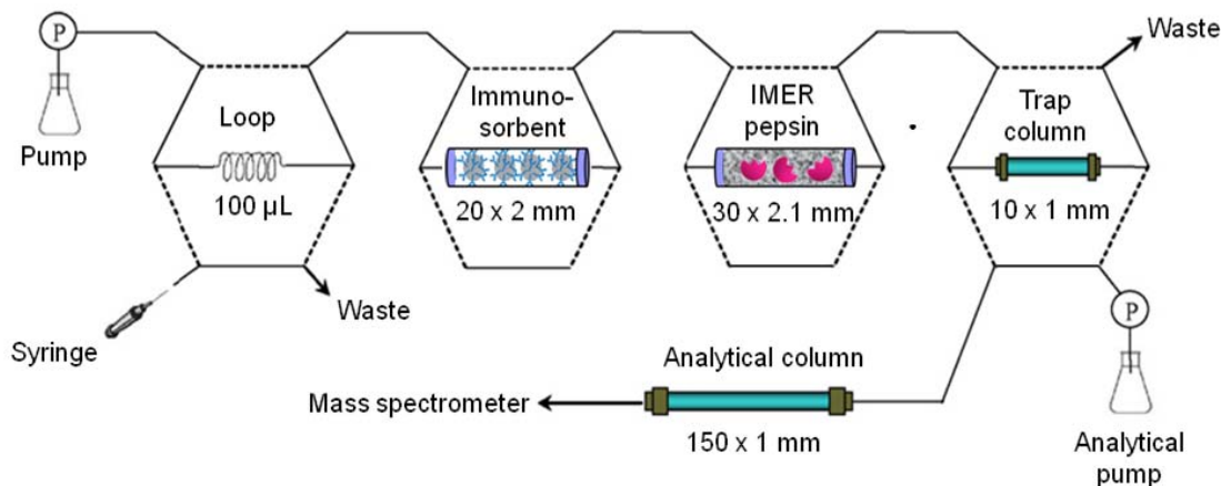
Fig. 1 Set-up used for the on-line immunoextraction of HuBuChE in 50 µL of plasma, followed by pepsin digestion on IMER and analysis of HuBuChE peptides by microLC/MS 2
