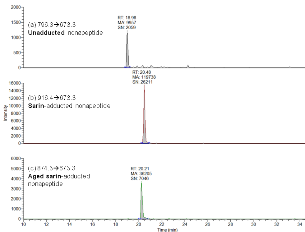
Fig. 3 MRM chromatograms of the intact nonapeptide (a), sarin-nonapeptide adduct (b) and aged sarin-nonapeptide adduct (c) obtained after immunoextraction on IS mAb2 SP of 50 \mu\text{L} of HuBuChE from plasma spiked with 100 \text{ ng}\cdot\text{mL}^{-1} of sarin, and digestion on IMER, followed by microLC/MS 2 analysis
