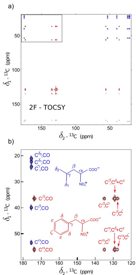
Figure 2. (a) Full two-field TOCSY spectrum of a mixture of 0.1 M leucine and phenylalanine in \text{D}_2\text{O} and (b) the region identified by a rectangle in (a) showing correlations between aliphatic (21–56 ppm), aromatic (128–135 ppm), and carboxylic (174–176 ppm) peaks. The peaks corresponding to leucine (blue) and phenylalanine (red) are distinguished by colours for clarity. All multiplets due to the homonuclear carbon-carbon couplings were masked in both dimensions to simplify the spectrum by multiplying the signals by an exponential function (line-broadening 40 Hz). All possible correlations were detected.
