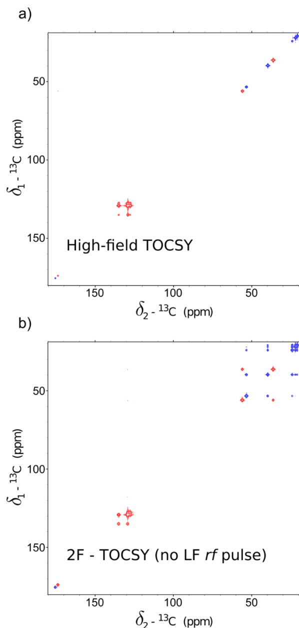
Figure 3. (a) Conventional TOCSY spectrum of the same sample as in Fig. 2 obtained at high field B_0^{\text{HF}} = 14.1 T. (b) Two-field TOCSY experiment acquired without any rf irradiation at low field. The peaks corresponding to the leucine (blue) and phenylalanine (red) molecules are distinguished by colours for clarity. Only cross-peaks close to the rf carrier frequency can be observed in (a). Only cross-peaks corresponding to spin networks that are strongly coupled at 0.33 T are detected in (b).
