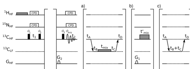
Figure 1. Pulse sequences employed for TOCSY experiments. The subscripts HF and LF designate channels at high field and low field, respectively. Non-selective \pi/2 pulses are denoted by filled rectangles. The grey rectangular box on the ^1\text{H}_{\text{HF}} channel depicts a 1.3 s WALTZ-16 composite-pulse irradiation [19] with an amplitude \gamma B_1^{\text{HF}}/(2\pi) = 714 Hz to allow the Overhauser effect to build up after a delay of 1 s between subsequent scans. WALTZ-16 composite pulse decoupling [20] with \gamma B_1^{\text{HF}}/(2\pi) = 1667 Hz is used for ^1\text{H}_{\text{HF}} and GARP-4 [27] with \gamma B_1^{\text{HF}}/(2\pi) = 1.04 kHz for ^{15}\text{N}_{\text{HF}} (rectangular boxes labelled CPD.) Three TOCSY experiments can be implemented: (a) with FLOPSY-16 [17] isotropic mixing (grey rectangle) with \gamma B_1^{\text{LF}}/(2\pi) = 1.5 kHz during t_{\text{mix}} = 31.28 ms. (b) high-field TOCSY experiment with FLOPSY16 [13] with \gamma B_1^{\text{LF}}/(2\pi) = 5.5 kHz applied at high field during t_{\text{mix}} = 16.96 ms. (c) Two-field TOCSY experiment without any rf -pulses at low field. The carbon-13 carrier frequency was placed at 100 ppm at both high and low fields. The phases cycles were \varphi_1 = \{x, -x\} , \varphi_2 = \{4x, 4(-x)\} , \varphi_3 = \{2x, 2(-x)\} , and \varphi_{\text{acq}} = \{x, -x, -x, x, -x, x, x, -x\} . Pulsed field gradients have smoothed rectangular shapes, with maximum amplitudes G_1 = 20 G/cm and G_2 = 17 G/cm, and durations of 0.5 ms. Sign discrimination in the indirect dimension is achieved by an alternation of \varphi_1 in the States-TPPI manner [21]. The spectra were acquired with N_1 = 230 t_1 time increments in the indirect dimension. The sample reached the low-field position in 120 ms and the return to the high-field position took 110 ms. Delays required because of hardware limitations prior to the sample transfer were t_A = 25 ms and t_C = 30 ms, respectively. The delays t_B = 10 ms and t_D = 300 ms allow possible vibrations to be attenuated.
