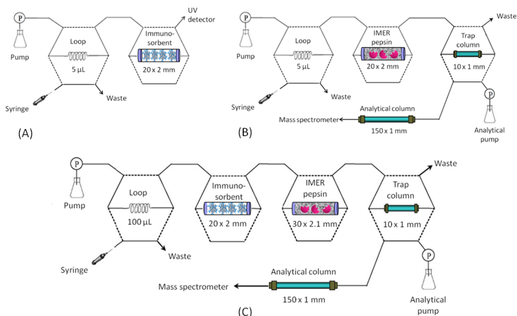
Fig. 1. Set-up used for the immunoprecipitation of 5 \mu\text{L} of HuBuChE solution on the immunosorbents (A). Set-up used for the on-line pepsin digestion of 5 \mu\text{L} of HuBuChE solution on IMER and its analysis by microLC/MS (B). Set-up used for the on-line immunoprecipitation, followed by pepsin digestion and analysis of HuBuChE in 50 \mu\text{L} of plasma (C). The trap column concentrated the peptides.
