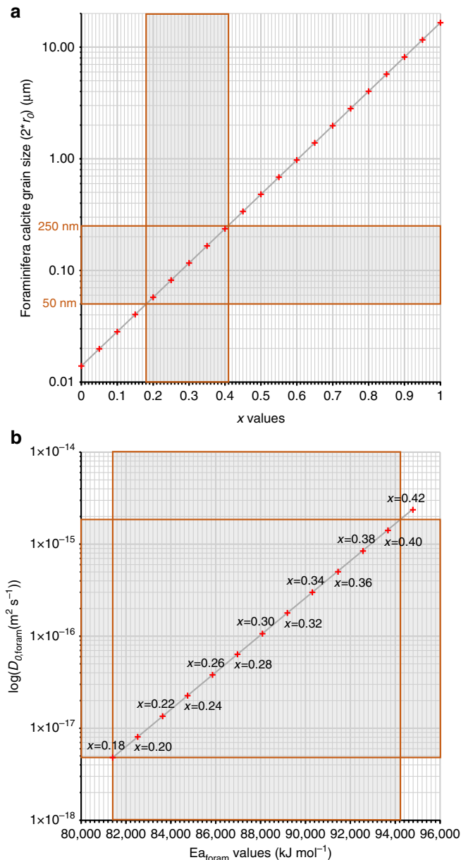
Fig. 5 Determination of the E_{a, \text{foram}} and D_{0, \text{foram}} values for the oxygen solid-state diffusion in foraminifera calcites. a Foraminifera calcite grain sizes ( 2 \cdot r_0 values) obtained using Eq. (15) for the different x values (Eq. (16)). b D_{0, \text{foram}} and E_{a, \text{foram}} values obtained using Eq. (16) for the different x values
