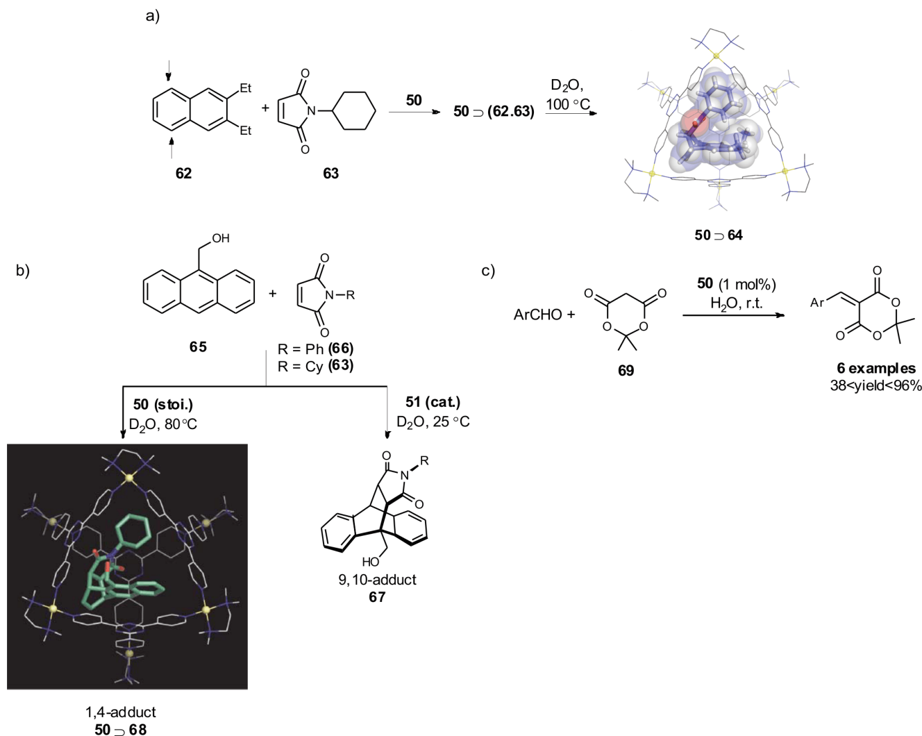
Fig. 14 a) Reaction between N -cyclohexylmaleimide 63 and 2,3-diethylnaphthalene 62 selectively yields the adduct 64 . Crystal structure of 50 \rightleftharpoons 64 . (The X-ray structure is reprinted with permission from ref. 398. Copyright 2010. American Chemical Society.) b) The Diels–Alder reaction between 65 and 66 is catalysed by 51 and yields the 9,10-adduct 67 . The reaction between 65 and 63 with a stoichiometric amount of 50 yields the 1,4-adduct. c) The Knoevenagel condensation of Meldrum's acid 69 with various aldehydes is catalysed by 50 but not by 51 . Refs: see the text.
