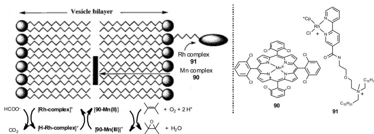
Fig. 21 Supramolecular cytochrome P450 mimic developed by Nolte et al. DODAC , DPPC , DPPA ( L - \alpha -dipalmitoylphosphatidic acid) and DHP are the surfactants used for the formation of the vesicles. Ref: see the text. See Fig. 18 for the name and formulas of DODAC , DPPC and DHP . (The schematic representation of the P450 mimic is reprinted with permission from ref. 498. Copyright 1998. John Wiley and Sons).
