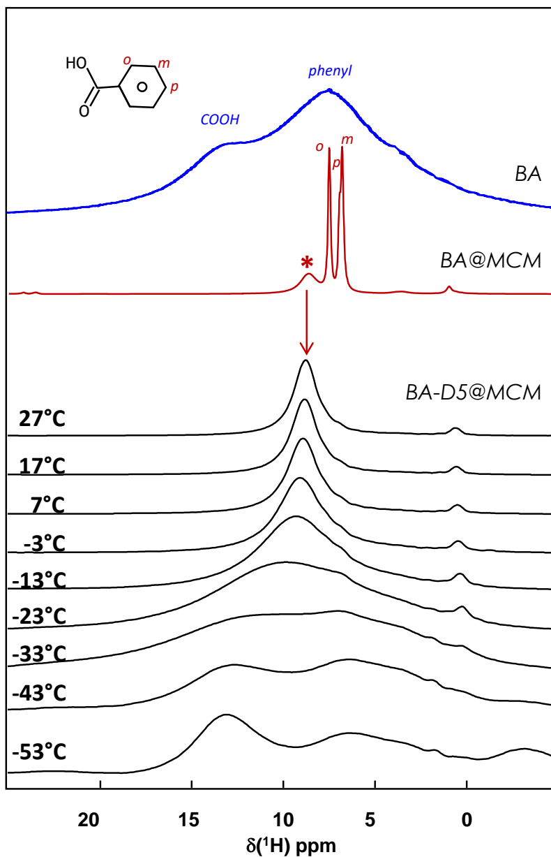
Figure 2. ^1\text{H} MAS NMR spectra of BA ( B_0 = 7\text{ T} , \nu_{\text{MAS}} = 14\text{ kHz} ), BA@MCM ( B_0 = 7\text{ T} , \nu_{\text{MAS}} = 14\text{ kHz} ) and BA-D5@MCM recorded at variable temperatures ( B_0 = 7\text{ T} , \nu_{\text{MAS}} = 5\text{ kHz} ). Asterisk denotes the specific resonance followed through ^1\text{H} MAS NMR variable temperature experiments (see text for details). Resonances assignment for BA and BA@MCM is given in the Figure.
