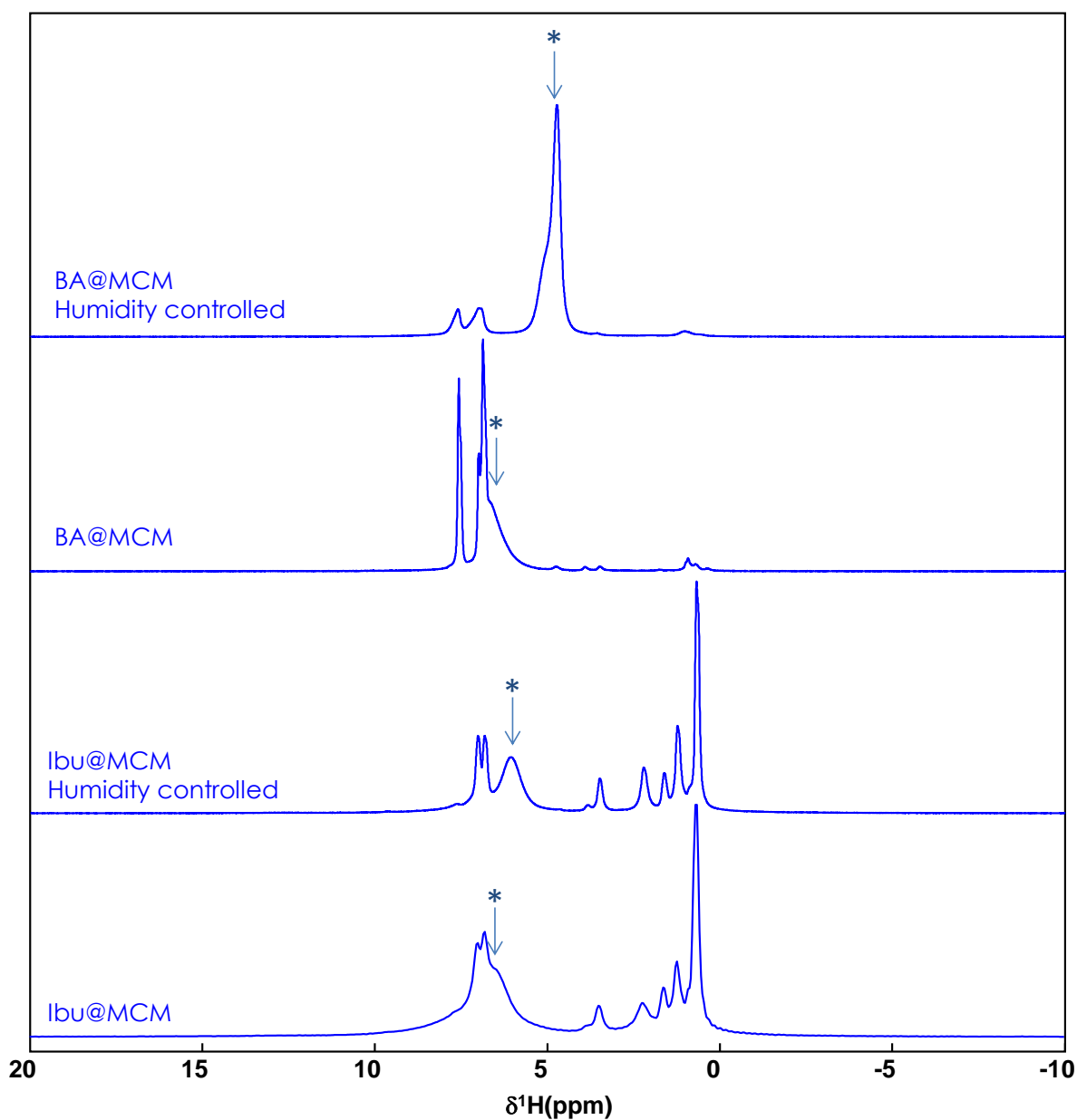
Figure 4. ^1\text{H} MAS NMR spectra of BA@MCM and Ibu@MCM without and with one night of equilibration in a 75% humidity controlled atmosphere. Asterisks denote the \text{H}_2\text{O} -COOH exchange resonance. B_0 = 7\text{ T} , \nu_{\text{MAS}} = 14\text{ kHz} .
