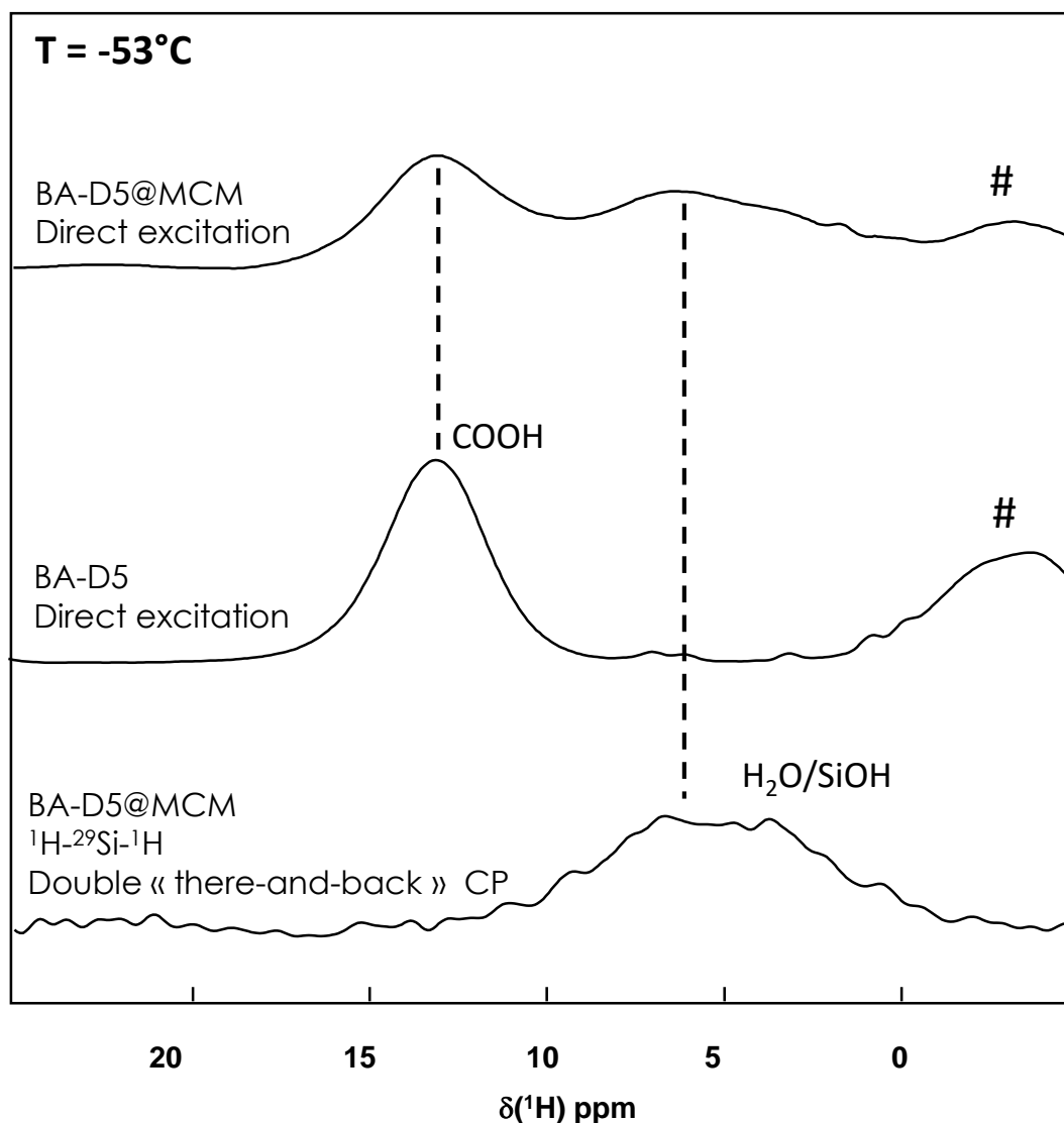
Figure 3. Low temperature ( T = -53^{\circ}\text{C} ) ^1\text{H} MAS NMR spectra of BA-D5@MCM (direct excitation), BA-D5 (direct excitation) and BA-D5@MCM ( ^1\text{H} - ^{29}\text{Si} - ^1\text{H} Double “there and back” CP). # denotes spinning side bands. B_0 = 7\text{ T} , \nu_{\text{MAS}} = 5\text{ kHz} .
