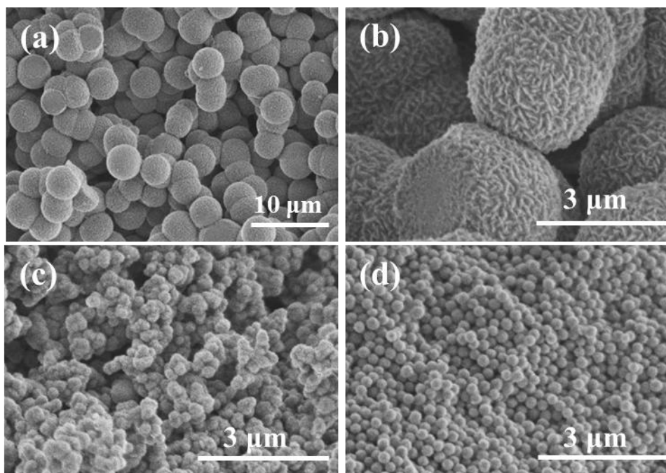
Figure 1: SEM pictures of the synthesized ZnS. (a, b) Microspheres of ZnS with an inorganic capping agent ( \text{K}_2\text{S}_2\text{O}_7 0.1% w/v), (c) Nanoparticles of ZnS (no capping agent), (d) Nanospheres of ZnS with an organic capping agent (PVP, 2% w/v).
