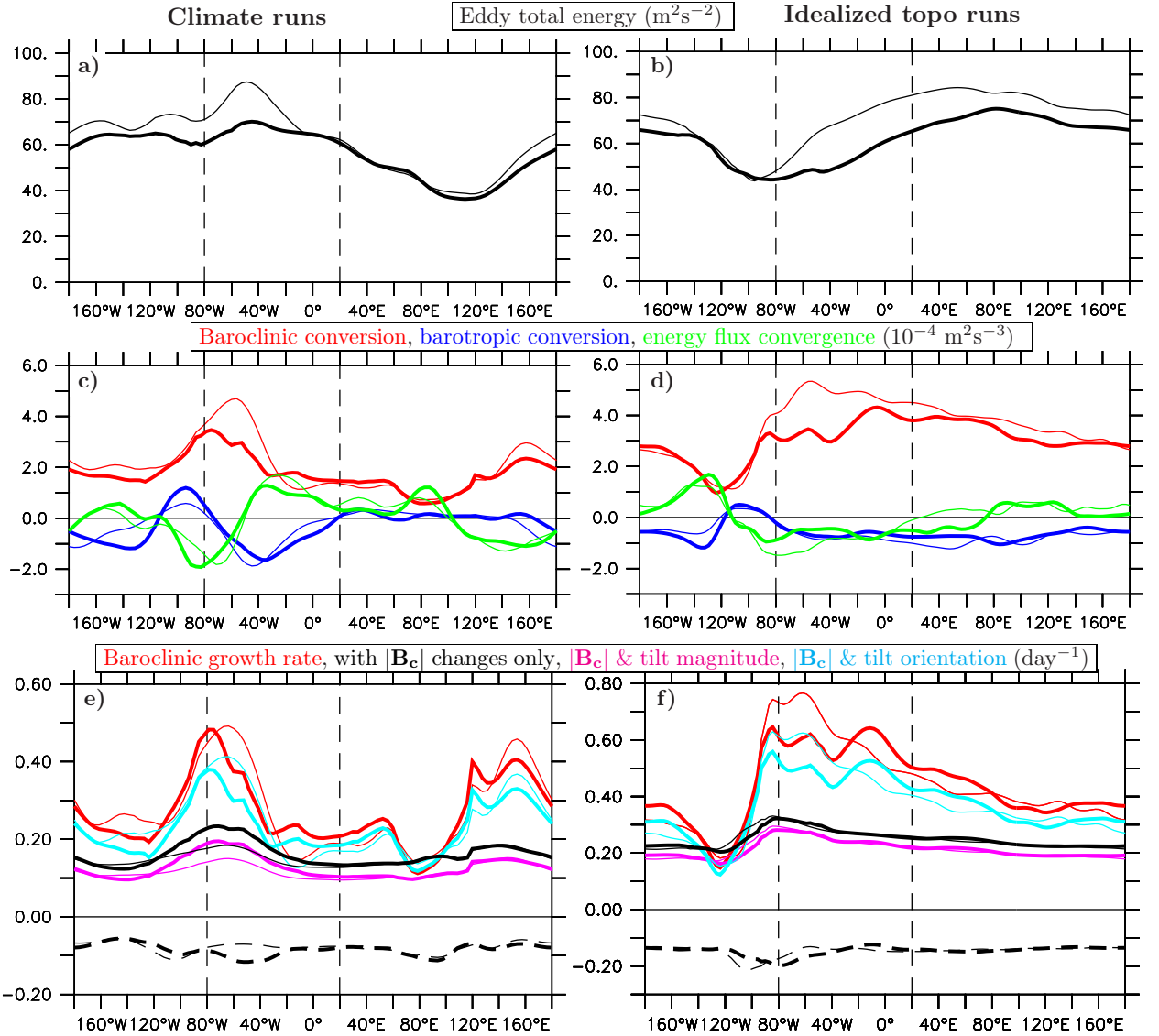
FIG. 3. ETE budget for (left column) the climate runs and (right column) the idealized topography runs where the thin and thick lines correspond to PI and LGM conditions respectively. (a), (b) ETE averaged between 250 and 850 hPa and between 25°N and 65°N. (c), (d) Baroclinic conversion (red), barotropic conversion (blue) and energy flux convergence (green). (e), (f) Baroclinic growth rate (red), with |\mathbf{B}_c| changes only (black), both |\mathbf{B}_c| and tilt magnitude changes (magenta) and both |\mathbf{B}_c| and tilt orientation changes (cyan). All the quantities have been averaged between 250 and 850 hPa and between 25°N and 65°N. The dashed black lines correspond to the residual term, the third term on the rhs of Eq.(7). The vertical dashed lines indicate the North Atlantic sector between 80°W and 20°E.
