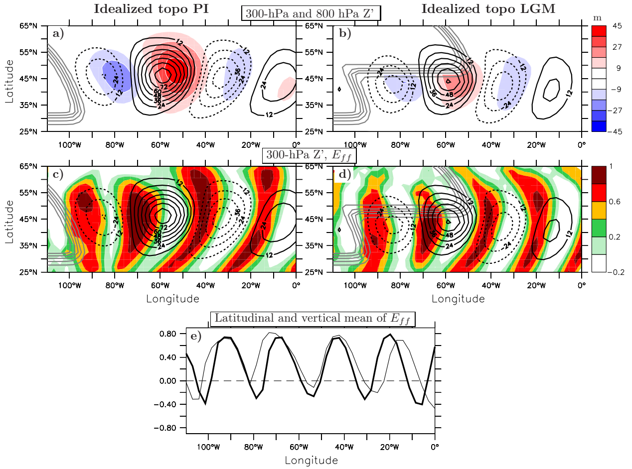
FIG. 9. As in Fig. 6 but for the simulations forced with (left) idealized Rockies (right) idealized LGM topography.
