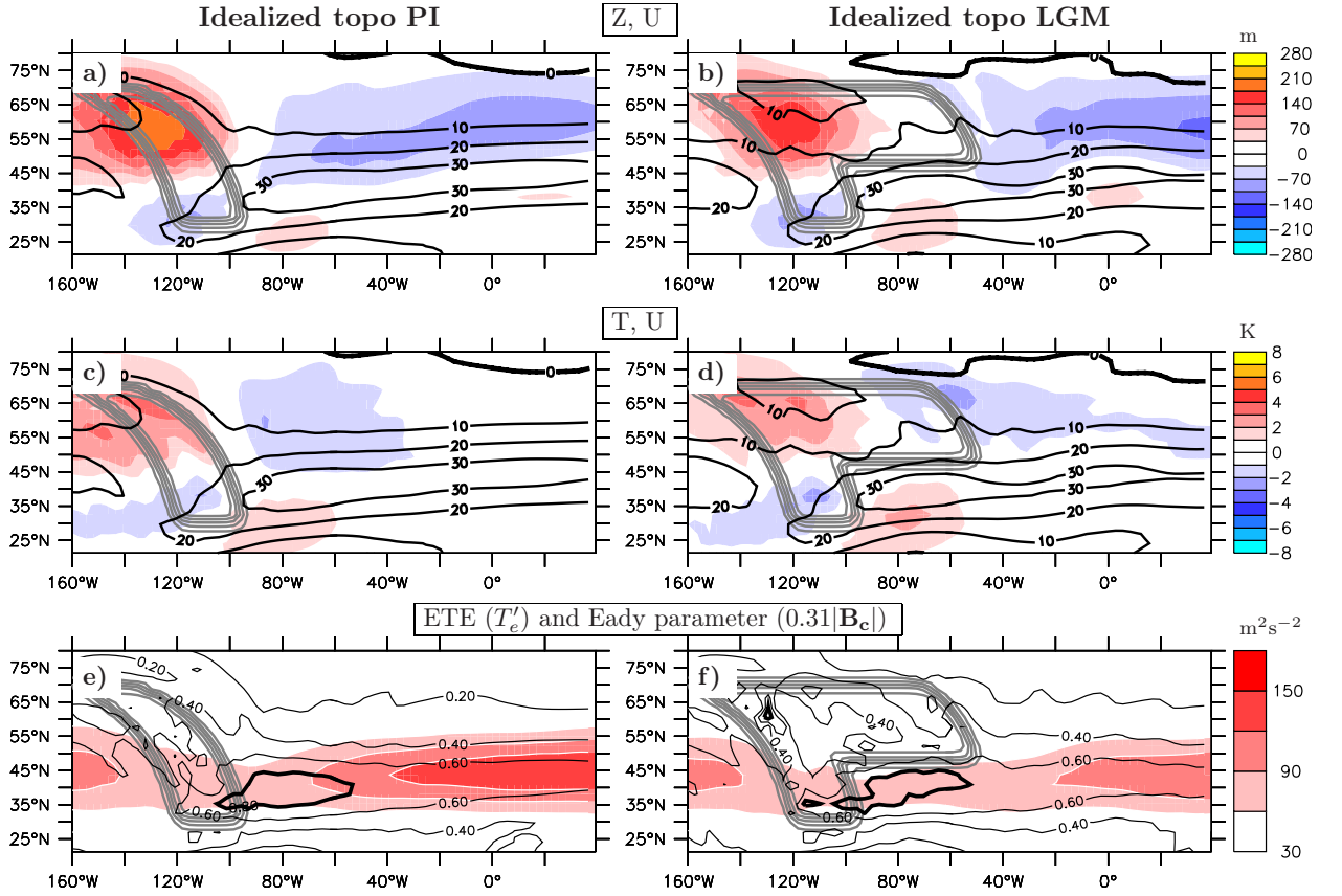
FIG. 2. As in Fig. 1 but for the simulations forced with (left) idealized Rockies (right) idealized LGM topog- raphy.
