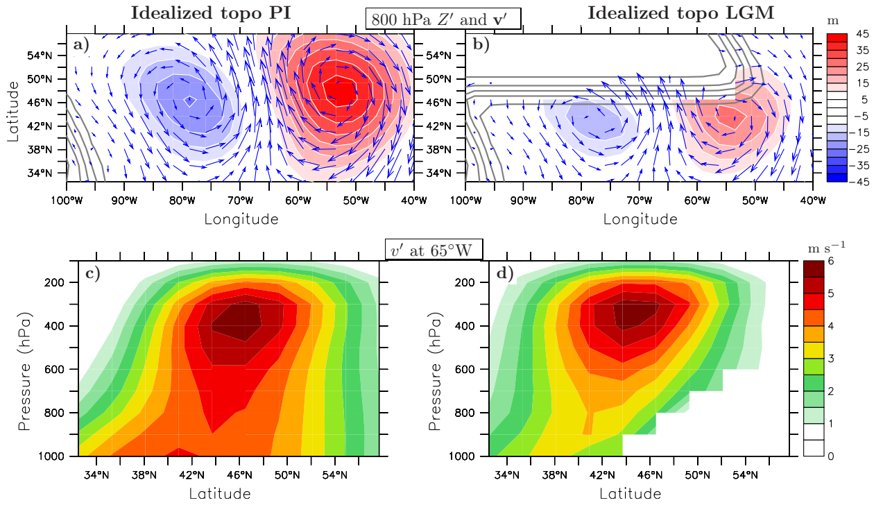
FIG. 10. As in Fig. 7 but for the simulations forced with (left) idealized Rockies (right) idealized LGM topography.
