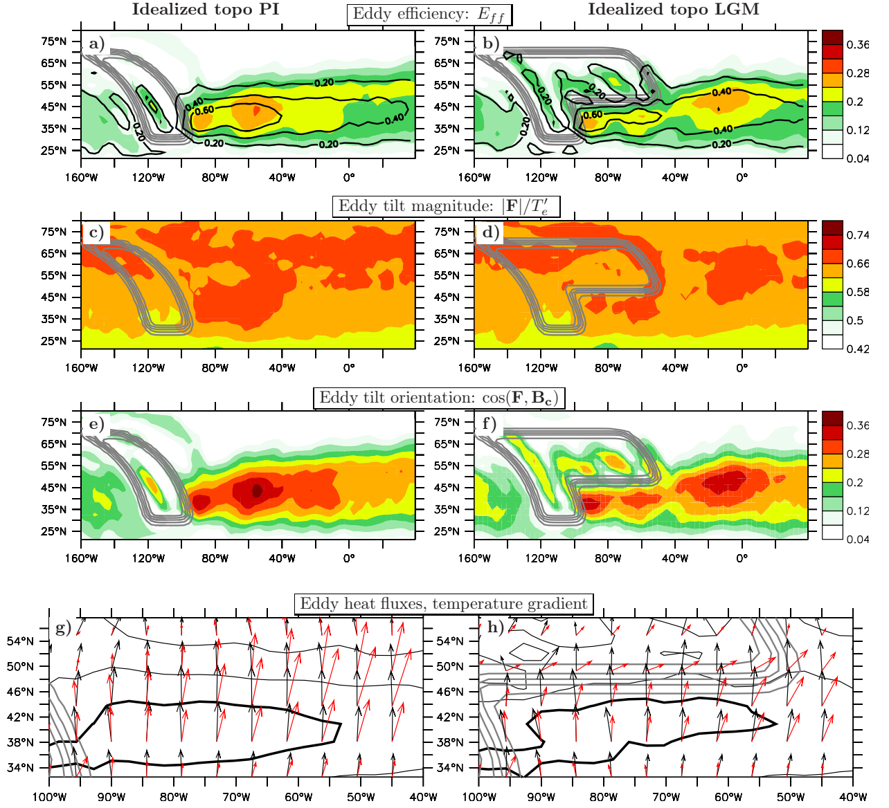
FIG. 5. As in Fig. 4 but for the simulations forced with (left) idealized Rockies (right) idealized LGM topography.
