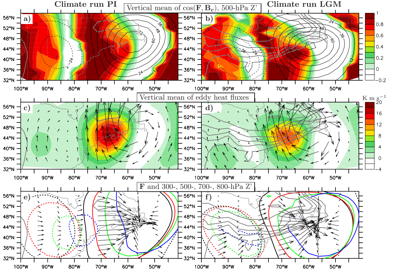
FIG. 8. Same regression as in Fig. 6 for (left) the PI climate run and (right) the LGM climate run. The regressed variables are (a), (b) the vertically-averaged tilt orientation \cos(\mathbf{F}, \mathbf{B}_c) (shadings) and 500-hPa perturbation geopotential height Z' (contours; int:12 m s -1 ); (c), (d) the vertical averages of the heat fluxes (vectors) and their meridional component (shadings); (e), (f) the vertically-averaged \mathbf{F} vector (arrows) and the 20-m contour of eddy geopotential height Z' at 300 (black), 500 (red), 700 (green), 850 hPa (blue). Grey contours correspond to the height of the orography (int: 500 m, starting from 500m).
