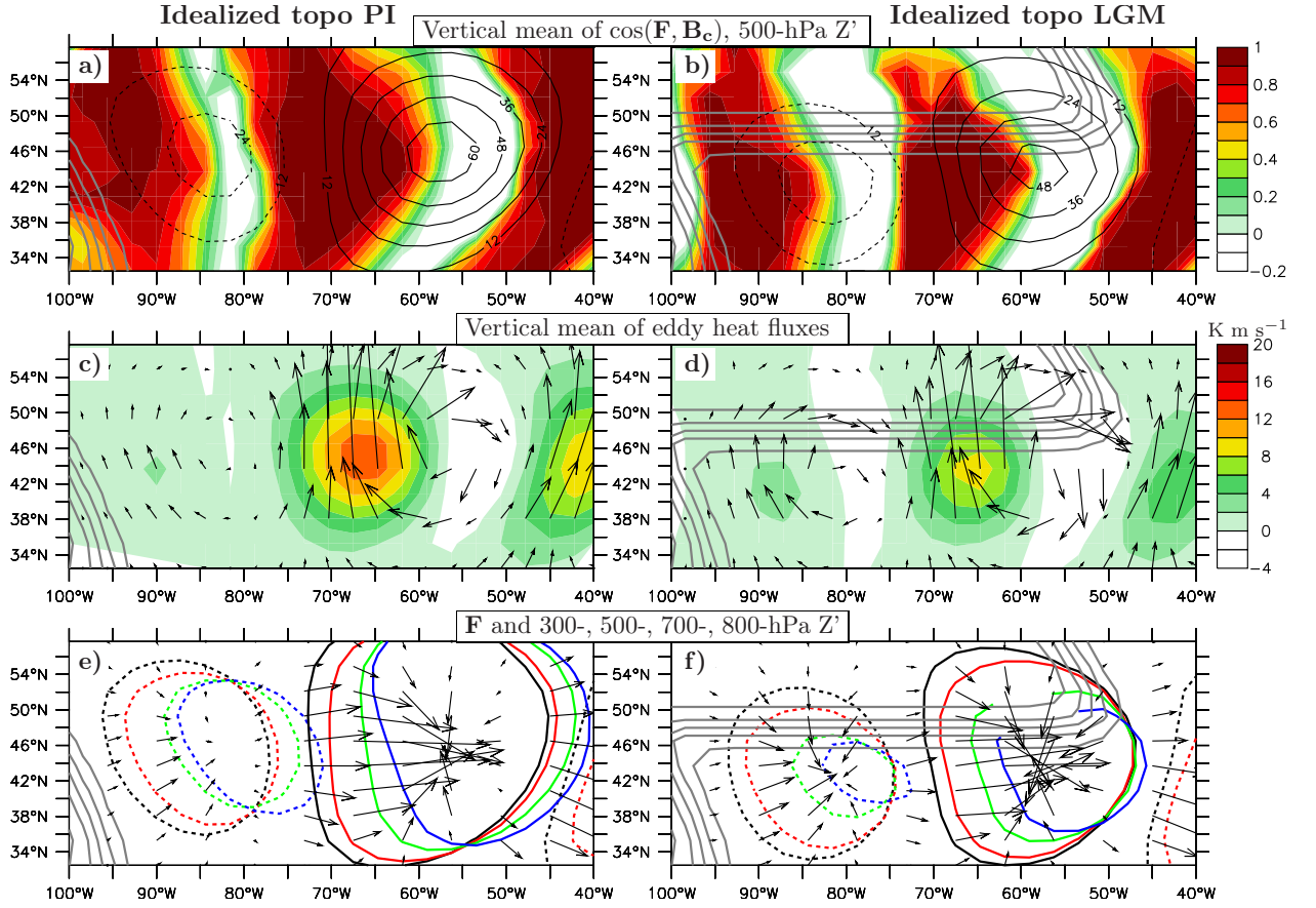
FIG. 11. As in Fig. 8 but for the simulations forced with (left) idealized Rockies (right) idealized LGM topography.
