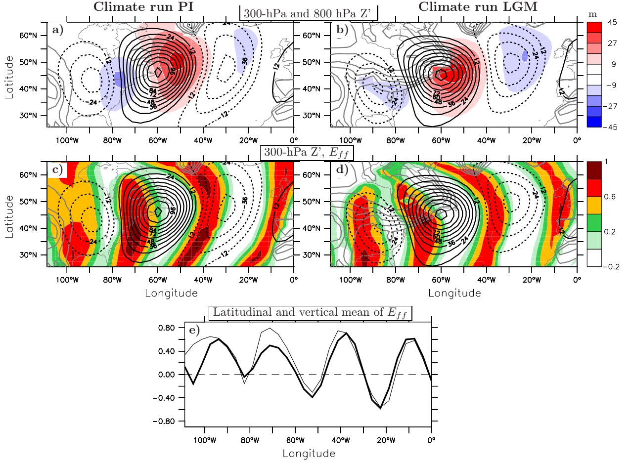
FIG. 6. One-point regression based on 300-hPa high-pass geopotential height Z' at 60^\circ\text{W} , 45^\circ\text{N} for (left) the PI climate run and (right) the LGM climate run; (a), (b) 300-hPa Z' (contours; int: 12 m) and 800-hPa Z' (shadings; int: 9 m); (c), (d) 300-hPa Z' (contours; int: 12 m) and associated vertically-averaged efficiency E_{ff} (shadings; int: 0.05); (e) vertical and latitudinal average of the regressed efficiency E_{ff} for PI (thin line) and LGM (thick line). In (a)-(d), grey contours correspond to the height of the orography (int: 500 m, starting from 500m).
