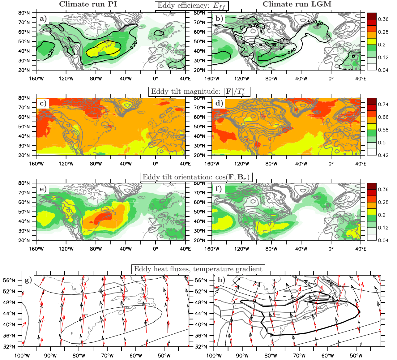
FIG. 4. Time mean and vertical average (250-850 hPa) of various quantities involved in the baroclinic conversion term for (left) the PI climate run and (right) the LGM climate run: (a),(b) the baroclinic growth rate |\mathbf{B}_c|E_{ff} (contours; int: 0.2 \text{ day}^{-1} ) and the eddy efficiency E_{ff} (shadings); (c),(d) the tilt magnitude |\mathbf{F}|/T'_e ; (e), (f) the tilt orientation \cos(\mathbf{F}, \mathbf{B}_c) ; (g), (h) the eddy heat fluxes (red) and minus the temperature gradient (black), and Eady growth rate 0.31|\mathbf{B}_c| (contours; int 0.2 \text{ day}^{-1} with 0.8 \text{ day}^{-1} in thick contour). Grey contours correspond to the height of the orography (int: 500 m, starting from 500m).
