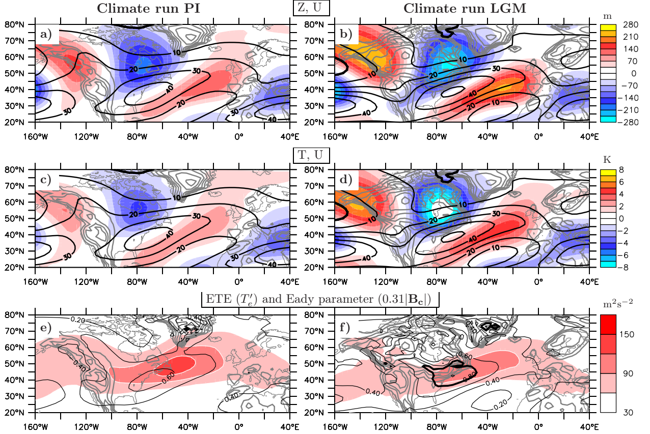
FIG. 1. (a), (b) Climatology of the anomalous (deviation from the zonal mean) geopotential height (shadings; int: 35 m) and the zonal wind at 300 hPa (contours; int: 10 \text{ m s}^{-1} for positive values only and the zero line is in bold); (c), (d) Climatology of the anomalous (deviation from the zonal mean) temperature at 500 hPa (shadings; int: 1 K) and the zonal wind at 300 hPa (contours; int: 10 \text{ m s}^{-1} for positive values only and the zero line is in bold); (e), (f) Eady growth rate 0.31|\mathbf{B}_c| (contours; int 0.2 \text{ day}^{-1} with 0.8 \text{ day}^{-1} in thick contour) and high-pass eddy total energy averaged between 250 and 850 hPa (shadings; int: 30 \text{ m}^2 \text{ s}^{-2} ). (Left column) PI and (right column) LGM simulations. Grey contours correspond to the height of the orography (int: 500 m, starting from 500m).
