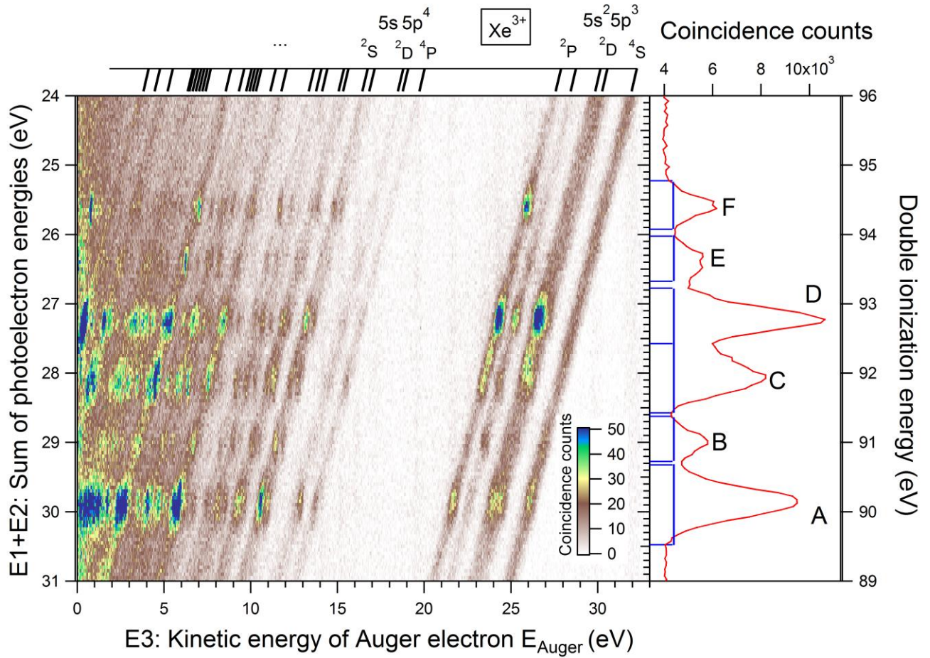
Figure 4: Experiment with HERMES setup. Core valence double photoionization of neutral Xe atoms at 120 eV photon energy. Left: Coincidence map for events where three electrons have been detected in coincidence. The coincidence map shows the energy correlations between the sum of the kinetic energies of two of them ( E1+E2 ) -y axis- versus the kinetic energy of the third one E3 -x axis-. The right panel shows the projection of the coincidence map on the y axis, revealing the \text{Xe}^{2+} 4d^{-1}5p^{-1} states. The rectangles indicate the peak boundaries selected for the analysis of the Auger spectra in Figure 6 and 7.
