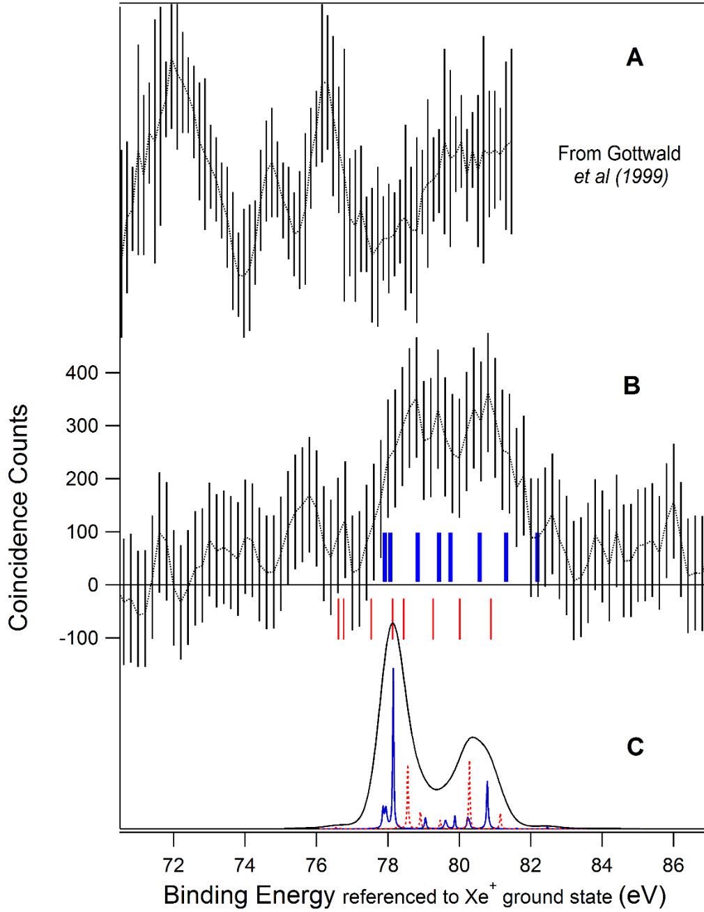
Figure 3: (B, middle) Experiment with MAIA setup: 4d photoelectron spectrum from photoionization of \text{Xe}^+ ions with 120.7 eV photons (middle). It is compared to the previous experiment by Gottwald et al [4] at h\nu = 103.3 eV (A, top). The broad blue and thin red vertical bars indicate the expected energy positions for the \text{Xe}^+ 5\text{p}^{-1} ({}^2\text{P}_{3/2}) \rightarrow \text{Xe}^{2+} 4\text{d}^{-1}5\text{p}^{-1} and the \text{Xe}^+ 5\text{p}^{-1} ({}^2\text{P}_{1/2}) \rightarrow \text{Xe}^{2+} 4\text{d}^{-1}5\text{p}^{-1} transitions, respectively; the transition energies are estimated using the 4\text{d}^{-1}5\text{p}^{-1} binding energies of Kivimäki et al [25]. The blue (solid) and red (dotted) curves in the bottom graph C show the calculated \text{Xe}^+ ({}^2\text{P}_{3/2}) \rightarrow \text{Xe}^{2+} 4\text{d}^{-1}5\text{p}^{-1} and \text{Xe}^+ ({}^2\text{P}_{1/2}) \rightarrow \text{Xe}^{2+} 4\text{d}^{-1}5\text{p}^{-1} photoelectron spectra, respectively. The spectra are weighted according to the estimated \text{Xe}^+ ({}^2\text{P}_{3/2}) to \text{Xe}^+ ({}^2\text{P}_{1/2}) ratio in the ion beam. The lines are broadened by the Lorentzian lifetime contribution only. The black line shows the calculated spectrum with additional 700 meV Gaussian broadening to simulate the effect of the experimental resolution. Note that theoretical curves have been shifted by +2 eV to match the positions expected from reference [25] -vertical bars-.
