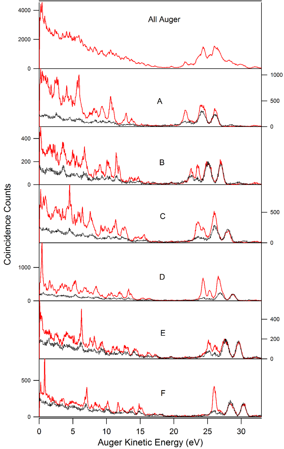
Figure 6: Experiment with HERMES setup. Auger spectra for the decay of each group of \text{Xe}^{2+} 4d^{-1} 5p^{-1} core-valence states defined in Figure 4 and 5. These Auger spectra are deduced from the experiment in Figure 4, as the intensity along each line associated to the corresponding group of core-valence states. The black dotted lines give the estimated background, obtained out of the core-valence peak region (see text for further explanation).
