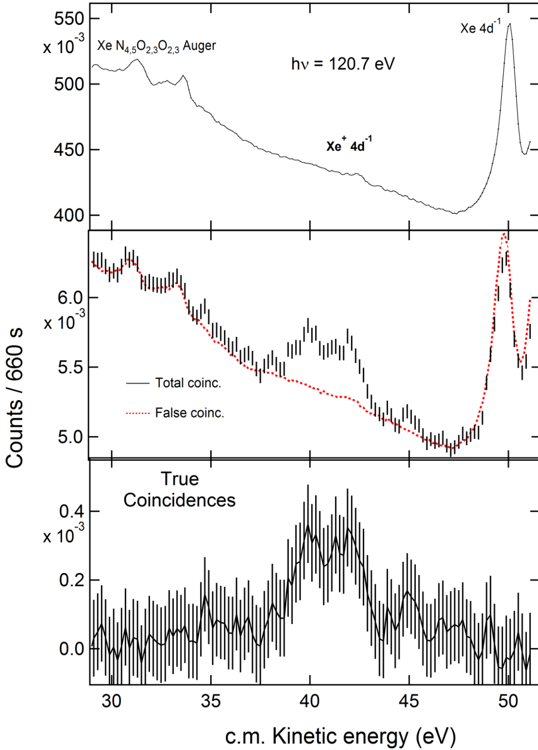
Figure 2: Experiment with MAIA setup on Xe + ions. Top: Raw photoelectron spectrum, represented as a function of the Center of Mass kinetic energy. Middle: Photoelectron spectrum in coincidence with Xe 3+ ions (points with error bars). The red (dotted) curve gives the estimated false-coincidence spectrum (see text for details). The bottom curve represents the resulting true coincidence spectrum (line with error bars). The photon energy was 120.7 eV and the spectral band pass was 110 meV. The error bars give the statistical uncertainty.
