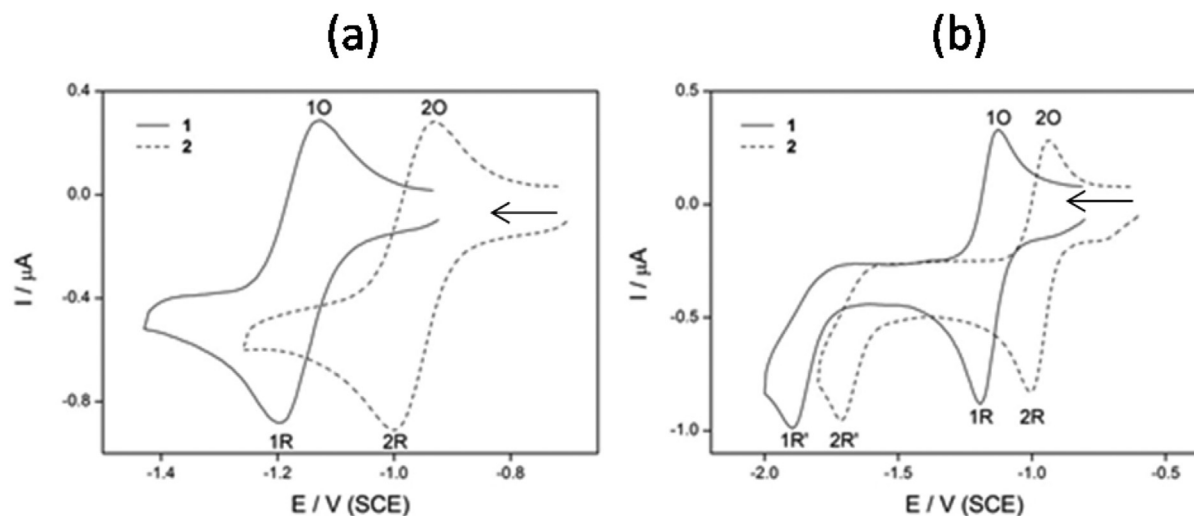
Fig. 1. Cyclic voltammograms of 1 (0.2 mM) and 2 (0.2 mM) in \text{MeCN}/[\text{TBA}][\text{BF}_4] (0.1 M), performed at a scan rate of 200 mV/s and at a glassy carbon electrode; (a) first reversible reduction process; (b) full scan.
