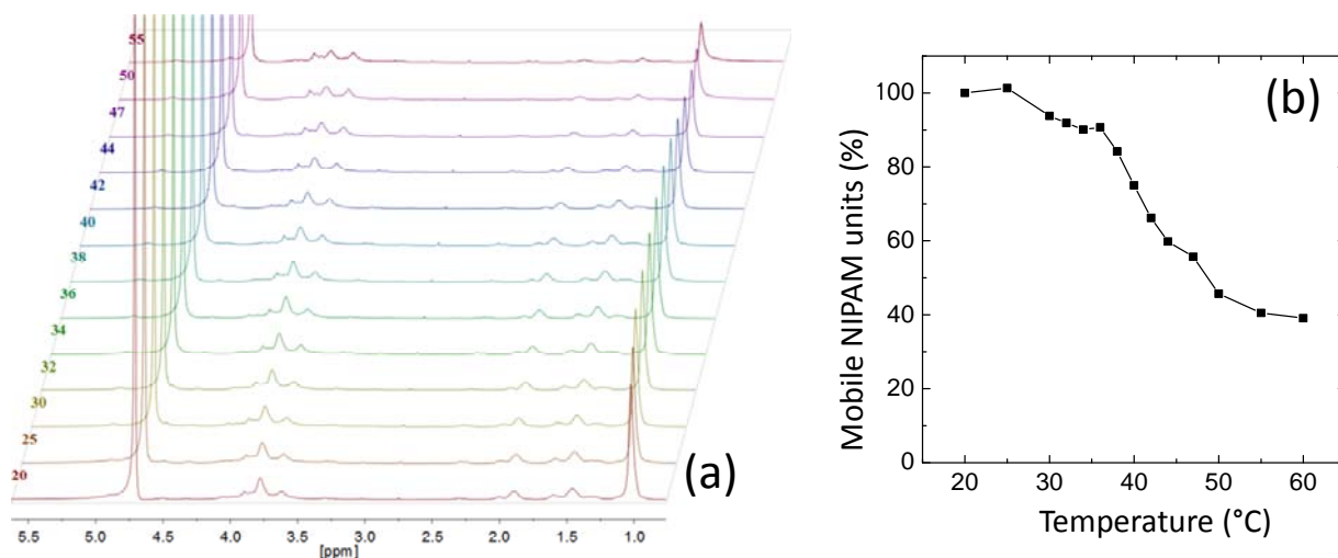
Figure 8. (a) Temperature variation of ^1\text{H} NMR spectrum of ALG-g-PNIPAM in D_2O solution ( C_p=5 wt%) and (b) temperature dependence of mobile NIPAM units within the graft copolymer.
