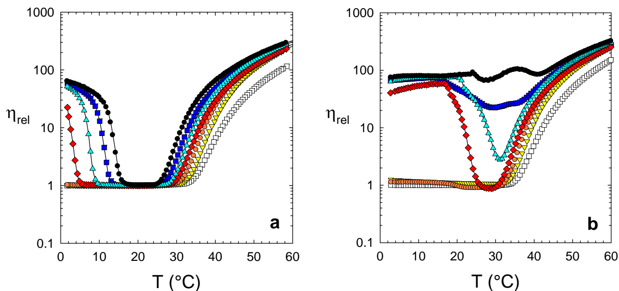
Figure 12. Temperature dependence ( a : cooling; b : heating) of the relative viscosity of ALG-g-PNIPAM aqueous solutions ( C_p = 5 wt%) prepared with KCl at different molar concentrations: 0 ( \square ); 0.2 ( \nabla ); 0.3 ( \circ ); 0.4 ( \diamond ); 0.5 ( \triangle ); 0.6 ( \blacksquare ) and 0.7 ( \bullet ).
