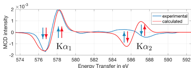
Fig. 17. Comparison the MCD CIE slices to visualise the inverted behaviour of K\alpha_2 MCD with respect to the K\alpha_1 emphasised with arrows indicating the local minima and maxima. The calculated MCD CIE slice is scaled to match the experimental intensity.
