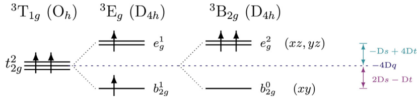
Fig. 6. Examples illustrating possible {}^3B_{2g} (D_{4h}) and {}^3E_g (D_{4h}) contributions in the compression case. The picture is restricted to the three t_{2g} (O_h) orbitals ( xy, xz, yz ) leaving the e_g (O_h) orbitals empty yielding a total of 9 micro states: 6 for {}^3E_g (D_{4h}) and 3 for {}^3B_{2g} (D_{4h}) .
