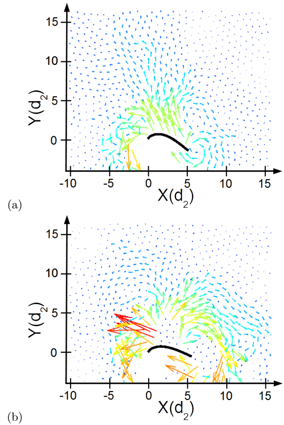
FIG. 4. Map of the displacement field of grains (amplified by a factor of 20) in the plate frame between 2 consecutive images for the loading and for the unloading phases of Fig. 3. The plate displacement U_0 between two consecutive images has been subtracted from each grain displacement. (a) Between the two images just before the unloading event (b) during the avalanche BC.
