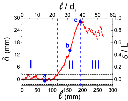
FIG. 6. Irreversible deflection of the bending fiber of length L = 3 cm in a granular medium of packing fraction \phi = 80.94\% for different penetration distances \ell . (a) \ell = 15.1 d_2 (b) \ell = 31.7 d_2 (c) \ell = 38.5 d_2 (d) Lateral deflection \delta of the free fiber extremity as a function of the penetration distance \ell . The horizontal dotted lines represent the maximum excursion of \delta during regime I. The three successive regimes I, II and III are separated by the vertical blue dotted lines.
