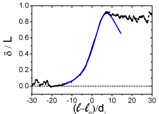
FIG. 13. Bending-induced compaction model (blue curve) superimposed on the experimental evolution of the averaged lateral deflection (black curve) as a function of the rescaled penetration distance with the same experimental parameters as in Fig. 7. The best A value obtained from the model is A=2200 \pm 750 Pa for this example.
