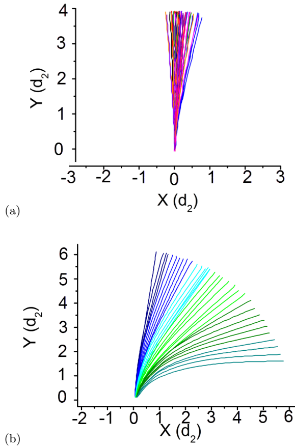
FIG. 2. (a) Fluctuations of an elastic beam of length L = 2 cm in a granular medium of packing fraction \phi = 80.94\% (jiggling regime). The clamping point of the fiber is located in (0,0) . The granular flow direction is along decreasing Y -axis. (b) Gradual bending of an elastic beam of longer length L = 3 cm (bending regime). The granular packing fraction is the same as in (a).
