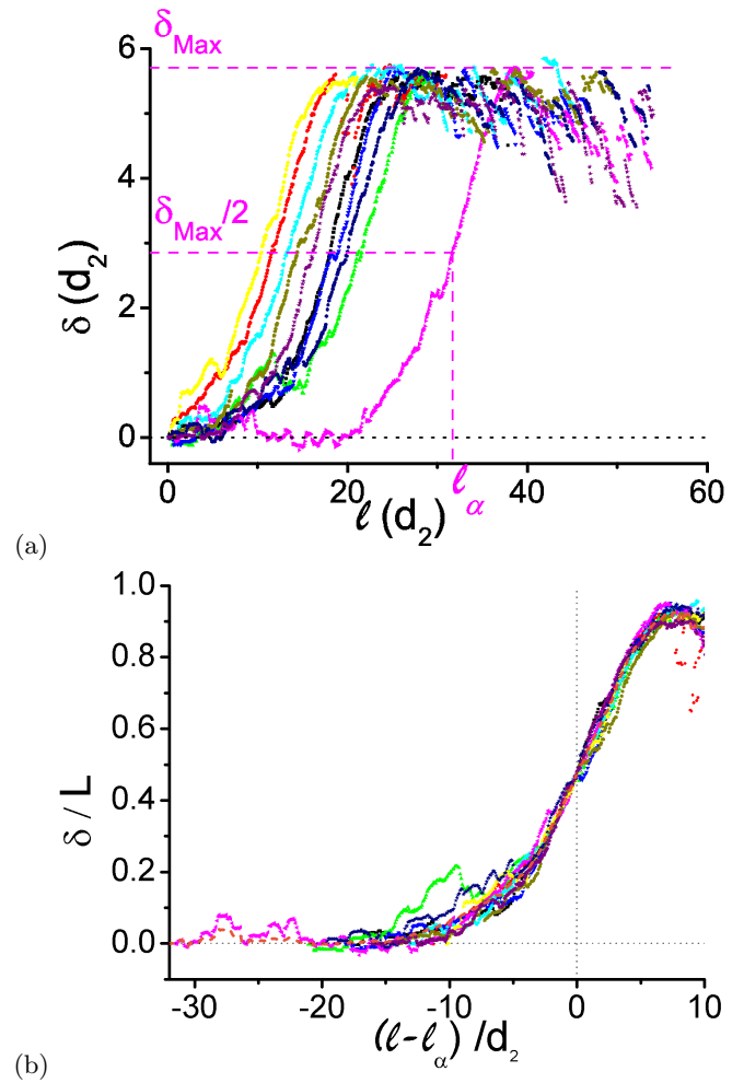
FIG. 7. (a) Lateral deflection \delta of the free extremity of the fiber as a function of the plate displacement (or penetration distance) \ell for 10 independent experiments performed with the same fiber length L = 3 cm and granular packing fraction \phi = 80.94\% . Both quantities are given in diameters of a large grain d_2 . All the 10 curves reach the same maximal value \delta_{Max} , with \ell_\alpha the penetration distance obtained for \delta_{Max}/2 . (b) Same curves as (a) expressed as a function of the reset penetration distance \ell - \ell_\alpha . The orange dash curve is the average over the different experimental curves.
