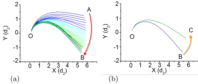
FIG. 3. Individual avalanche, loading and unloading of a fiber of length L = 3 cm in a granular medium of packing fraction \phi = 80.94\% for a highly bent configuration (regime III). (a) Successive fiber shapes during a loading phase (plate displacement of 2U_0 = d_2/6 between each fiber shape from A to B). (b) Unloading phase from B to C with a sudden elastic return of the fiber during one increment U_0 of plate displacement.
