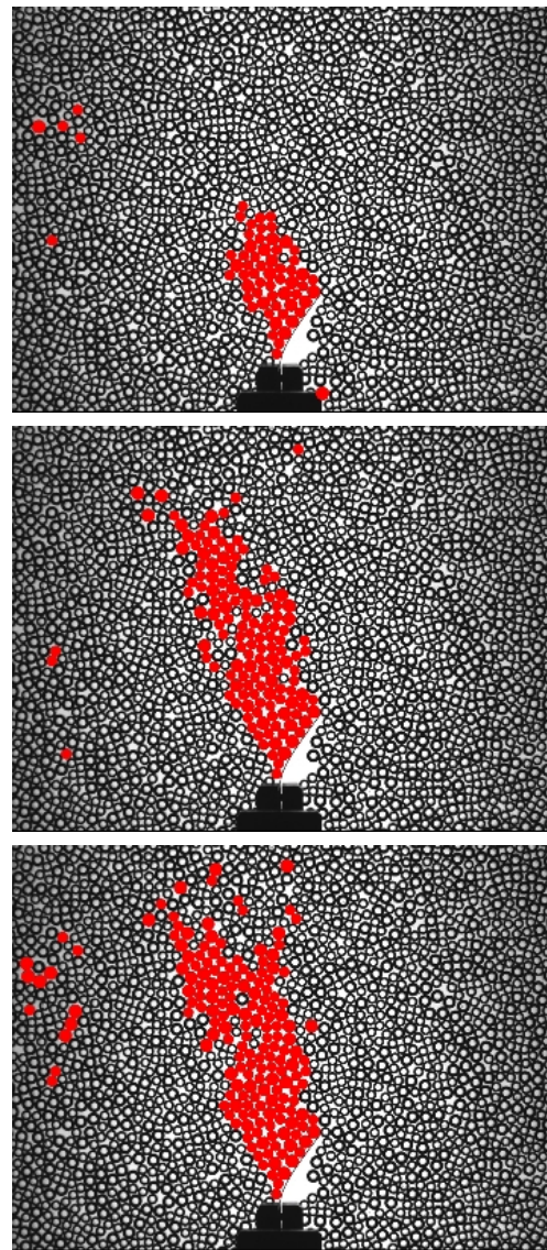
FIG. 10. Growth of a “cluster” of slow grains (red-labeled) for three successive images starting from a penetration distance \ell=24.1d_2 for a granular packing at \phi = 80.94\% and L = 3 cm.
