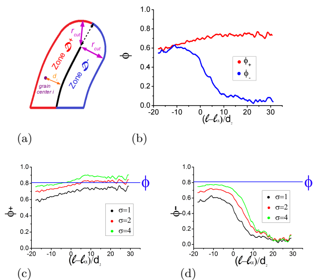
FIG. 11. Development of a packing fraction contrast between the two sides of the bending fiber. (a) Schematic diagram of the zones upstream and downstream of the fiber for calculation of \phi_+ and \phi_- . (b) Lateral packing fractions \phi_+ and \phi_- (sliding window averaged over 10 points and over 10 experiments) as a function of the rescaled penetration distance \ell - \ell_\alpha normalized by d_2 for a fiber length L = 3 cm in a granular medium with a macroscopic packing fraction \phi = 80.94\% (indicated by the blue horizontal line in (c) and (d)). Effect of the choice of the coarse-grained length scale \sigma on the calculation of (c) \phi_+ and (d) \phi_- .
