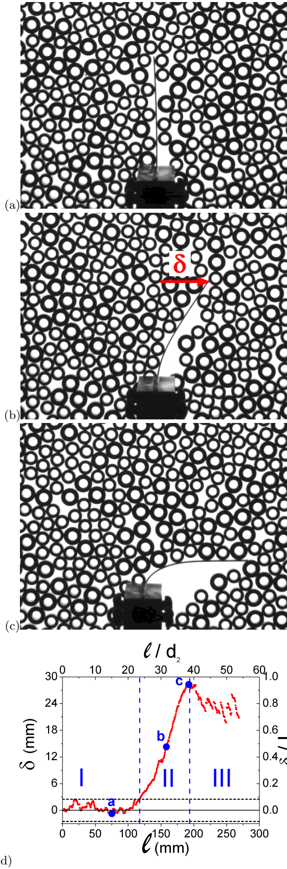
FIG. 6. Irreversible deflection of the bending fiber of length L = 3 cm in a granular medium of packing fraction \phi = 80.94\% for different penetration distances \ell . (a) \ell = 15.1 d_2 (b) \ell = 31.7 d_2 (c) \ell = 38.5 d_2 (d) Lateral deflection \delta of the free fiber extremity as a function of the penetration distance \ell . The horizontal dotted lines represent the maximum excursion of \delta during regime I. The three successive regimes I, II and III are separated by the vertical blue dotted lines.
