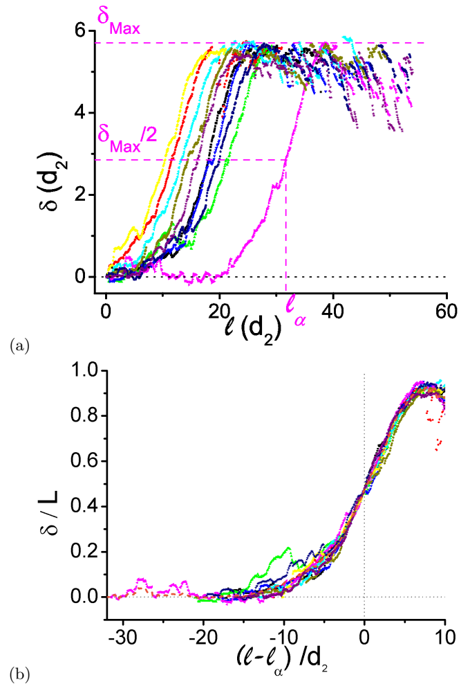
FIG. 7. (a) Lateral deflection \delta of the free extremity of the fiber as a function of the plate displacement (or penetration distance) \ell for 10 independent experiments performed with the same fiber length L = 3 cm and granular packing fraction \phi = 80.94\% . Both quantities are given in diameters of a large grain d_2 . All the 10 curves reach the same maximal value \delta_{Max} , with \ell_\alpha the penetration distance obtained for \delta_{Max}/2 . (b) Same curves as (a) expressed as a function of the reset penetration distance \ell - \ell_\alpha . The orange dash curve is the average over the different experimental curves.
