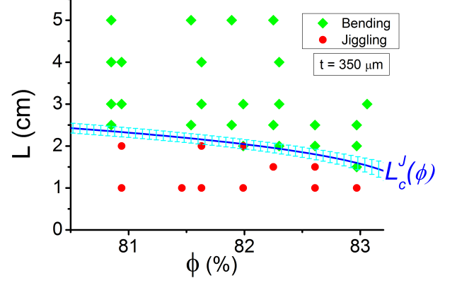
FIG. 5. Phase diagram in the plane L - \phi . Experiments vs prediction. The symbols represent the experiments performed by varying the fiber length L or granular packing fraction \phi with green diamonds for the bending regime and red circles for the jiggling regime. The blue curve is the predicted elasto-granular length from eq.(9) that separates the jiggling from the bending regimes with the associated error bars.
