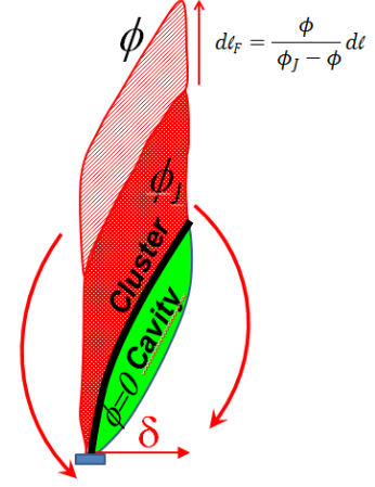
FIG. 12. Schematic diagram of the formation of a cluster at the jamming packing fraction \phi_J ahead of the fiber and a cavity empty of grains behind the fiber. Aggregation of grains in front of the cluster through the advance of a compaction front and cluster erosion through recirculations of grains (red arrows) on both sides of the flexible intruder. The rest of the granular layer is at the packing fraction \phi .
