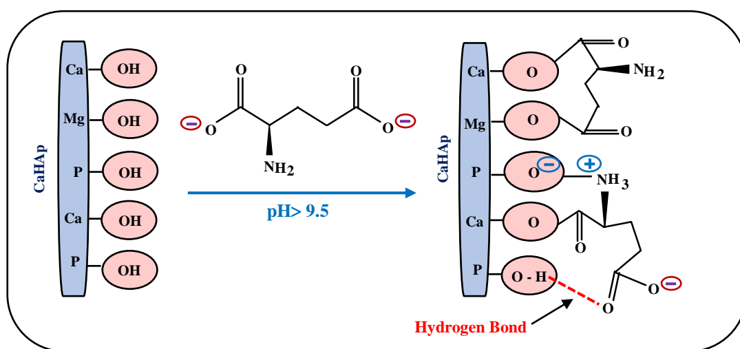
20 21 22 23 24 25 26 27 28 29 30 31 32 33 34 35 Scheme 1. Formation of Ca carboxylate salt leading to the grafting of glutamic on the CaHAp surface.
