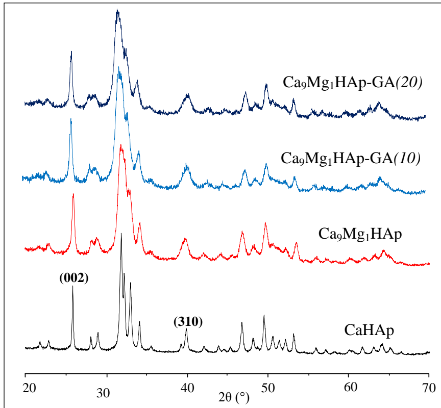
Fig. 5. X-ray diffractograms for CaHAp and \text{Ca}_9\text{Mg}_1\text{HAp} ungrafted and grafted.
