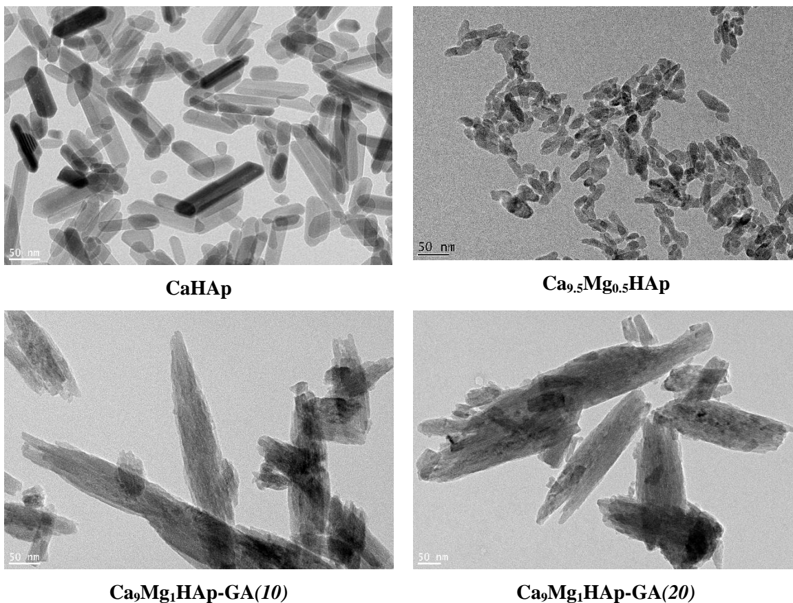
Fig. 7A. TEM images (Scale bars=50 nm) of CaHAp, Ca 9.5 Mg 0.5 HAp, Ca 9 Mg 1 HAp-GA(10) and Ca 9 Mg 1 HAp-GA(20).
