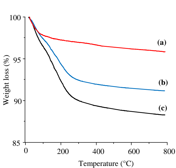
Fig. 1. TG plots; (a) Ca 9 Mg 1 HAp, (b) Ca 9 Mg 1 HAp-GA(10) and (c) Ca 9 Mg 1 HAp-GA(20).
