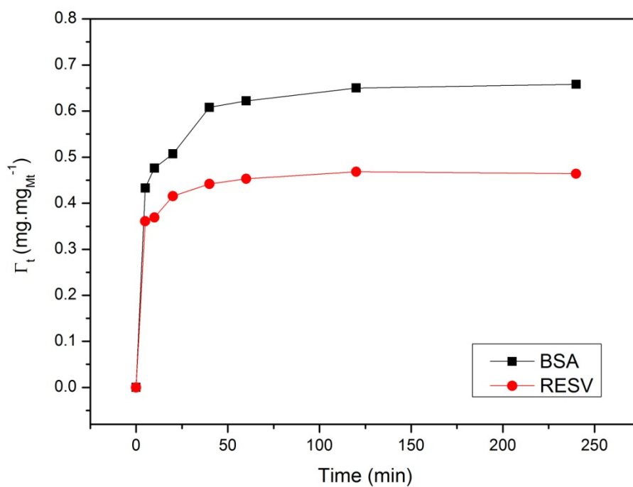
Figure 3 SI. Adsorption kinetics of BSA (black) and RESV (red) absorbed on montmorillonite. Experimental conditions: BSA (1.0 mg.mL -1 ), RESV (1.0 mg.mL -1 ), Mt (1.0 mg.mL -1 ) in a buffer phosphate at pH 4.5 and ethanolic solution in ratio of 25 %.
