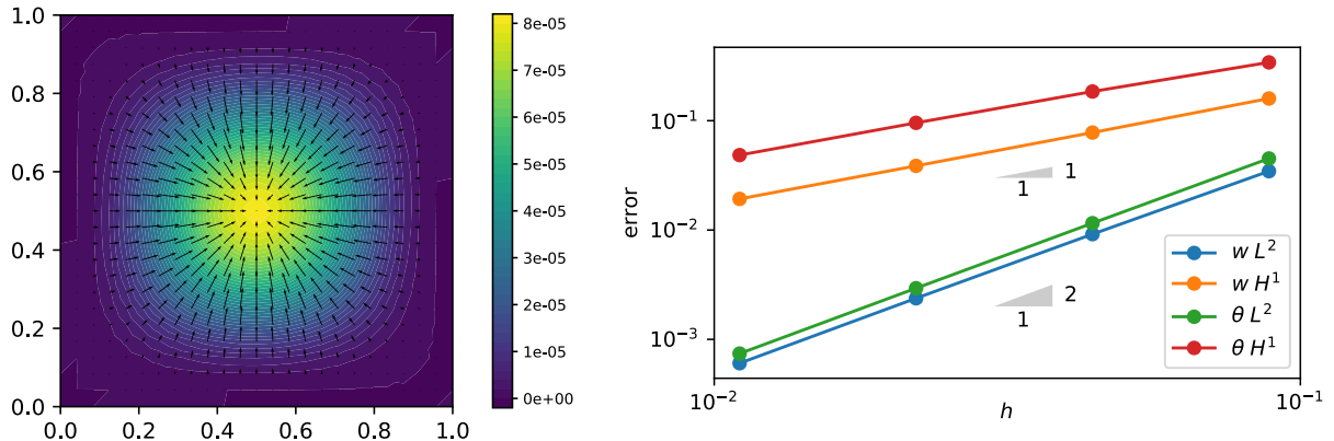
Figure 5: Chinosi clamped plate problem solved using Durán–Liberman element: Transverse displacements (scalar field, density plot) and rotations (vector field, quiver plot, 50% of points discarded) (left). Convergence to Chinosi analytical solution on sequence of uniformly refined meshes in H^1 and L^2 norms for t = 10^{-4} (right).
