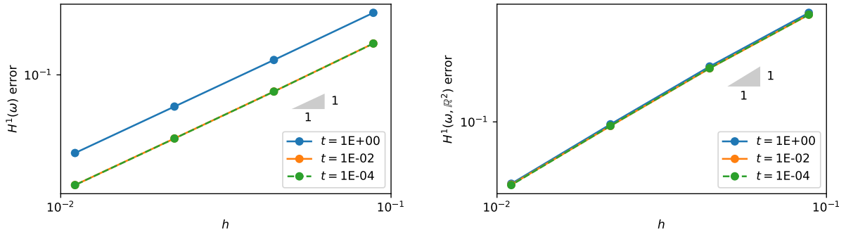
Figure 6: Convergence of Reissner-Mindlin problem discretised with Durán–Liberian element to Chinosi analytical solution for varying thickness parameter t . Left: Error for the transverse displacement w ( H^1 -norm) as a function of the mesh size h . Right: Error for the rotation field \theta ( H^1 -norm). In the latter case all lines lie on top of each other (convergence behaviour independent of t ). We achieve optimal convergence in all cases.
