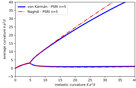
Figure 12: Lenticular orthotropic plate. Comparison of the results obtained with the von Kármán and the Naghdi models using the PSRI discretisation and an unstructured uniform mesh with n = 5 division along the radius. The results are for a^2/t = 100 and \nu = 0.3 .
