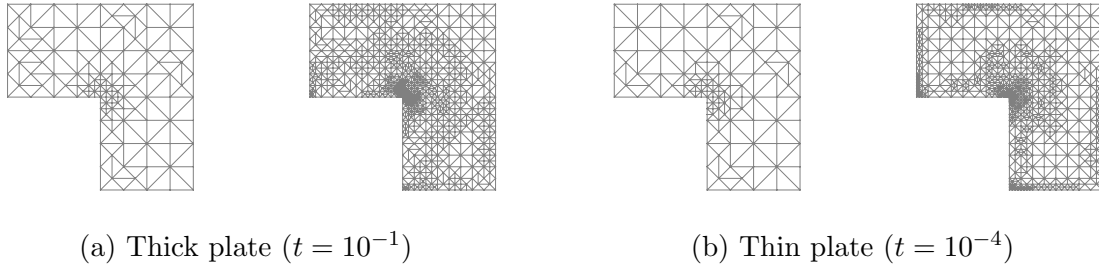
Figure 7: Meshes after adaptive remeshing at different refinement levels (3rd and 6th level) for thick and thin plates. The increased refinement on the free boundaries for thin plates capture the strong boundary layer effect as t \rightarrow 0 .
