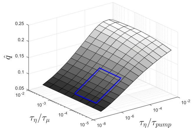
FIG. 3. Plot of dominant wave number \hat{q} = q^*R_{\text{eq}} of the instability against ratio of viscous to pumping time scales \tau_\eta/\tau_{\text{pump}} and ratio of viscous to permeable time scales \tau_\eta/\tau_\mu . All other parameters are the same as in Fig. 2. The blue rectangle indicates typical physiological parameters.
