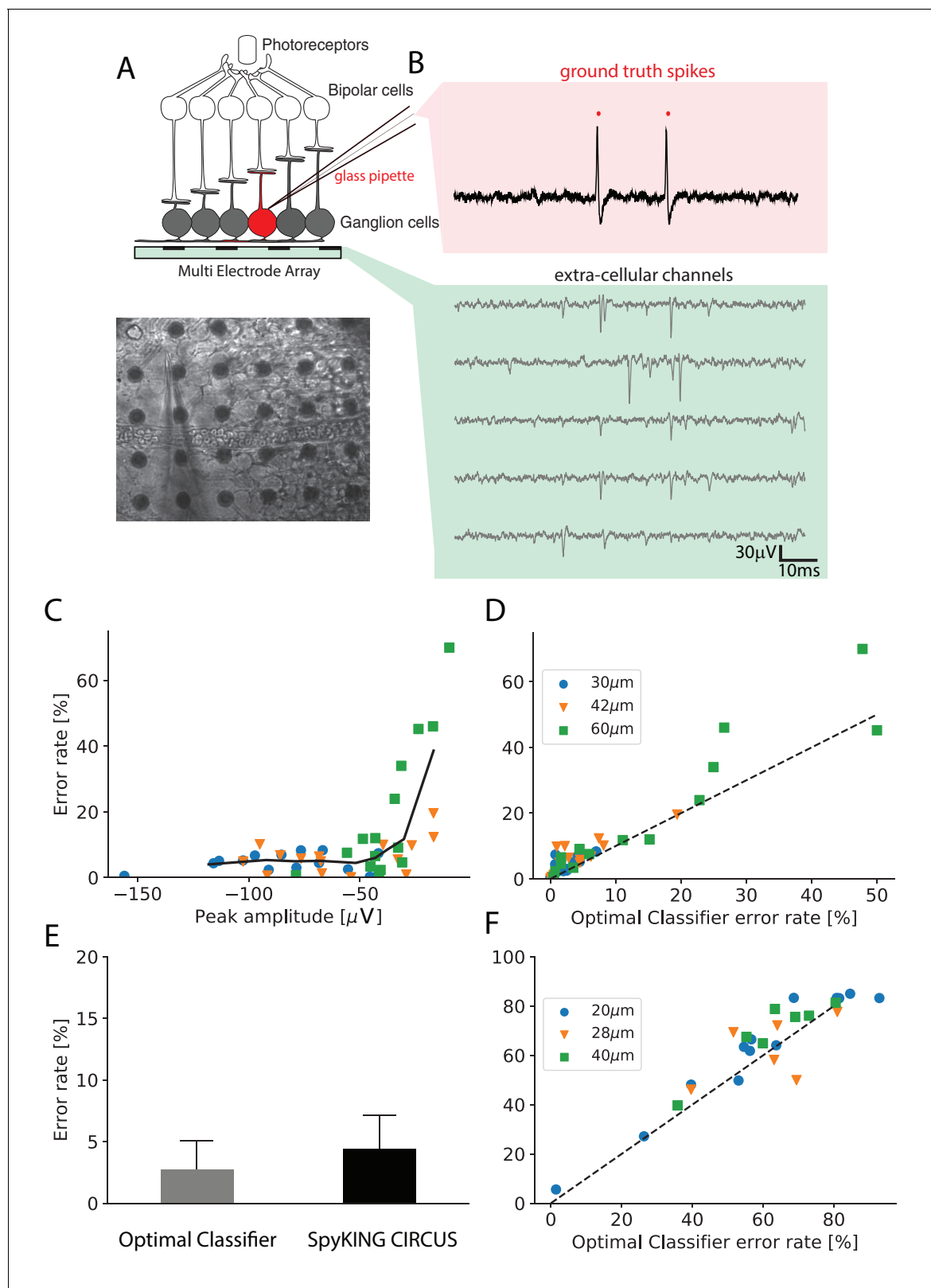
Figure 2. Performance of the algorithm on ground truth datasets. (A) Top: Schematic of the experimental protocol in vitro. A neuron close to the multi-electrode array (MEA) recording is recorded in loose patch. Bottom: Image of the patch electrode on top of a 252 electrodes MEA, recording a ganglion cell. (B) Top, pink box: loose patch recording showing the spikes of the recorded neuron. Bottom, green box: Extra-cellular recordings next to the loose patched soma. Each line is a different electrode (C) Error rate of the algorithm as function of the largest peak amplitude of the ground-truth spikes. Figure 2 continued on next page
