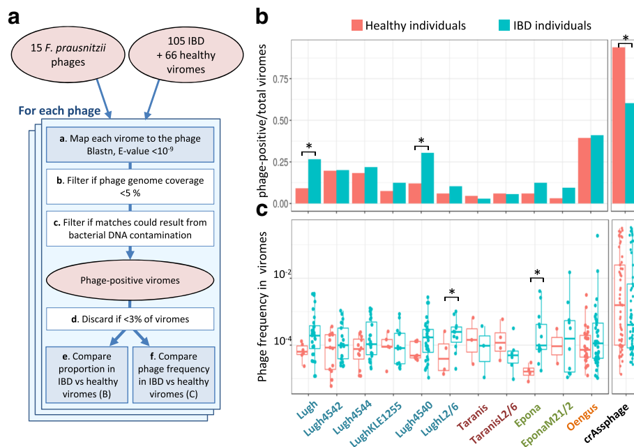
Fig. 5 F. prausnitzii phages in healthy versus IBD-diseased individuals from the dataset of Norman et al. [18]. a Workflow of the procedure. a To infer the presence of a phage in a given sample, virome reads were aligned to the phage genome, and hits showing greater than 75% identity were retained. b If hits of a given sample were concentrated on less than 5% of the phage genome, the sample was not considered further for this phage. c The number of hits was compared to the maximal theoretical number of hits that could result from the measured bacterial DNA contamination. If the number of hits was significantly higher, the sample was classified as phage-positive. d If phage-positive samples represent less than 3% of total samples, this phage was not further studied. e The proportion of phage-positive viromes is compared to IBD versus healthy viromes. f In phage-positive viromes, phage frequency is compared to IBD versus healthy samples. b Fraction of phage-positive samples according to the health status of individuals. Three phages are significantly more prevalent in IBD-diseased than in healthy individuals. The highly prevalent crAssphage was included as a positive control in the analysis. c Phage abundance (read frequency) in positive samples according to the health status of individuals. Two phages, Epona and LughL2/6, are significantly more abundant in IBD patients than in healthy individuals
