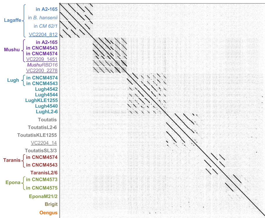
Fig. 1 Whole genome dot plot of the 23 F. prausnitzii prophages and 7 homologous sequences retrieved from the nr/nt database define six clades and two singletons (Brigit and Oengus, last lanes). Braces group similar prophages, which correspond to the same phage species found in different bacterial genomes. Names beginning “VC” (underlined) correspond to metagenomic viral contigs, and names in italic correspond to prophages in non- F. prausnitzii bacterial species
