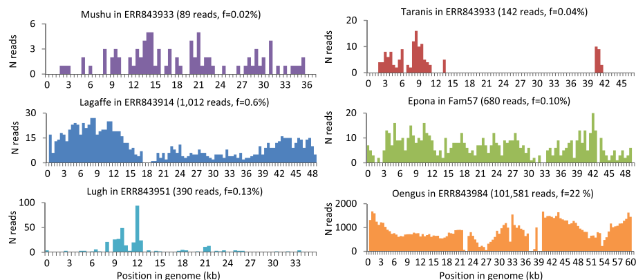
Fig. 4 F. prausnitzii phages are present in intestinal viromes. Read coverage for six type phages in samples with the best abundance and coverage from the datasets of Norman et al. [18] and Reyes et al. [52]. Number of aligned reads (ordinate) is represented as a function of position in the phage genome (abscissa). Phage name, virome name, total number of aligned reads, and ratio of aligned to total reads are shown for each panel
