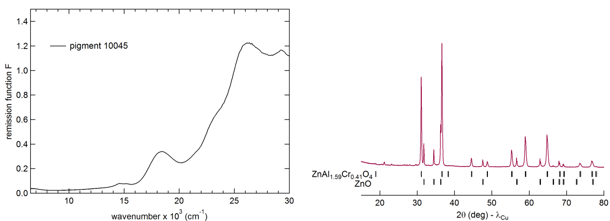
Figure 6: (left) Remission function F calculated from the diffuse reflectance spectra of pigment 10045. The high absorption in the near-UV region is due to the presence of ZnO, a semi conductor compound with a gap energy located at 26600 cm -1 . (right) XRD diagram of pigment 10045 with the main phases identified: ZnAl 1.59 Cr 0.41 O 4 and ZnO.
