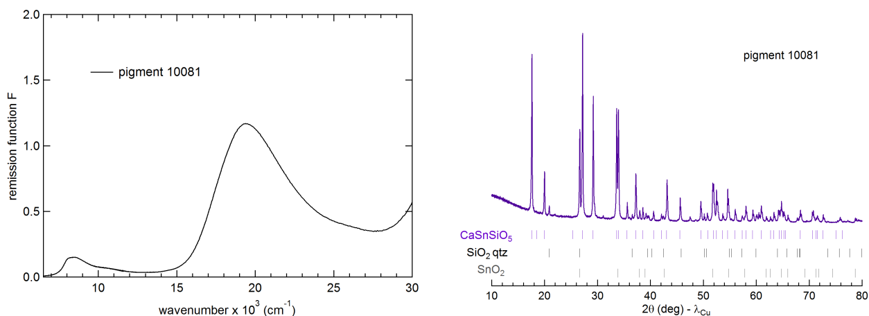
Figure 4: (left) Remission function F calculated from the diffuse reflectance spectra of pigment 10081 and (right) XRD diagram of pigment 10081 with the main phases identified: CaSnSiO 5 , SiO 2 quartz and SnO 2 .
