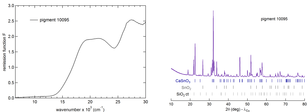
Figure 5: (left) Remission function F calculated from the diffuse reflectance spectra of pigment 10095 and (right) XRD diagram of pigment 10095 with the main phases identified: CaSnO 3 , SnO 2 and SiO 2 cristobalite.
