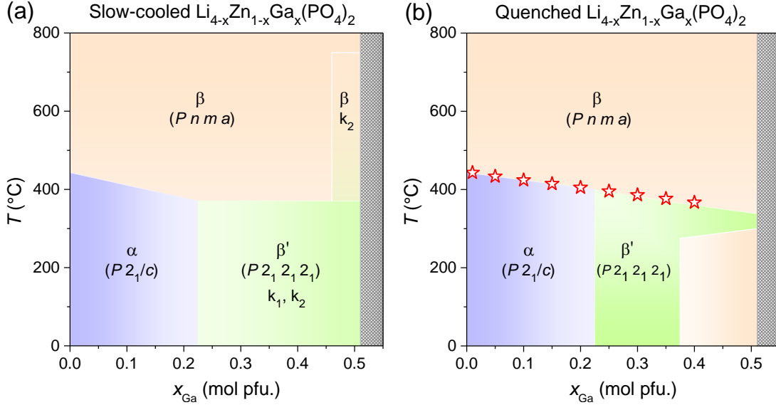
Figure 8. Temperature-Composition phase diagram of Li 4-x Zn 1-x Ga x (PO 4 ) 2 compounds, deduced from temperature-dependent X-ray diffraction and DSC experiments (red stars). The black shaded region indicates the presence of secondary phases for Ga contents above 0.5 mol pfu.
