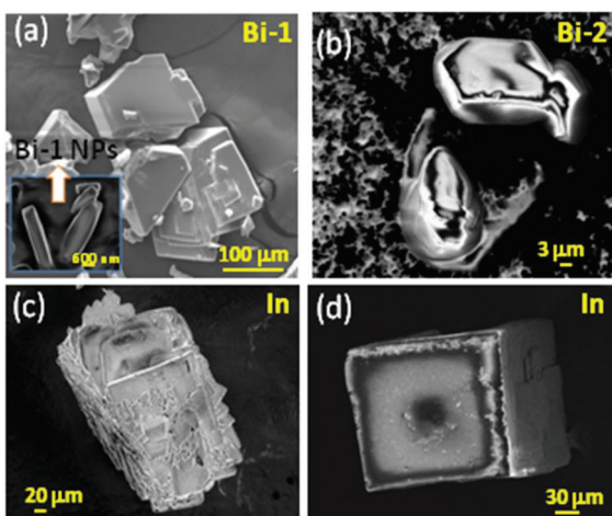
Fig. 1 Micrographs of (a) Bi-1, (b) Bi-2, and In-1 obtained (c) without and (d) with growth modulator.
