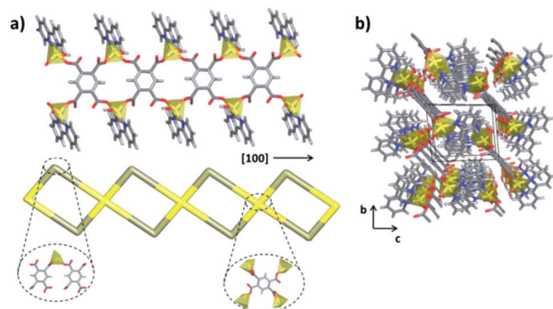
Fig. 4 (a) Polymeric chain and decorated simplified chain along the [1\ 0\ 0] direction and (b) crystal packing view into the bc plane of Zn-1 compound.
