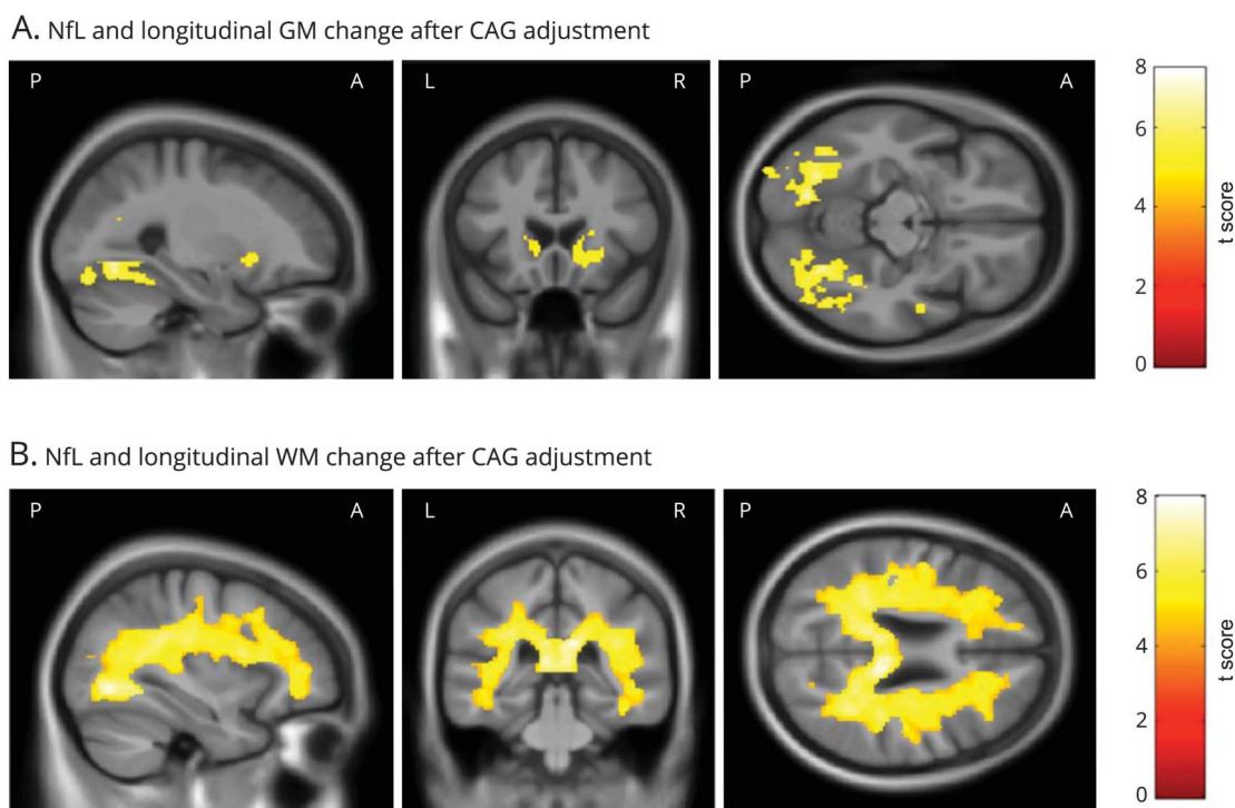
Figure 4 Significant associations between baseline NfL and change in GM and WM volume after adjustment for CAG
