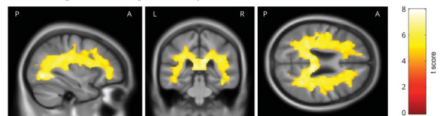
B. NfL and longitudinal WM change after CAG adjustment
