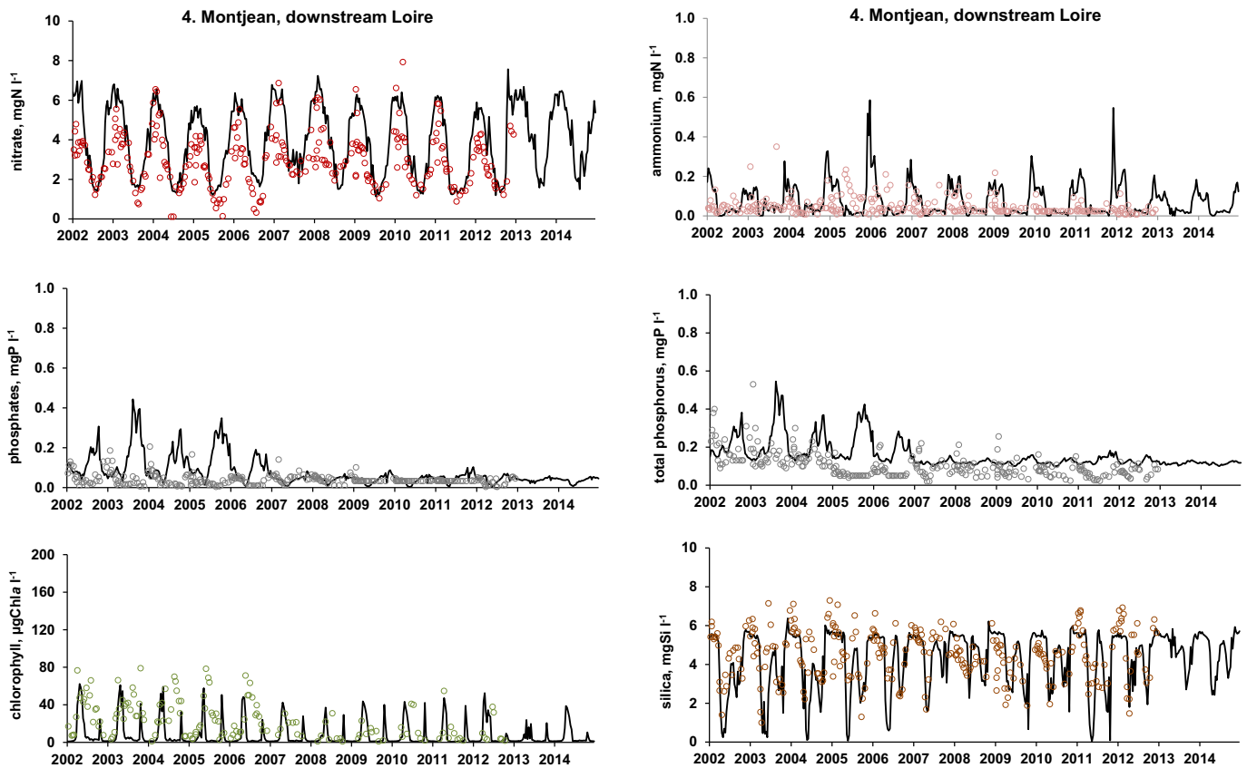
Fig. 5. Simulations by the Grafts-Senque-Riverstrahler model of the seasonal variations of major water quality variables at the outlet of the Loire River network (at Montjean-sur-Loire, namely Montjean). Comparison with observations for nitrate, ammonium, phosphates, total phosphorus, chlorophyll a and silica.
