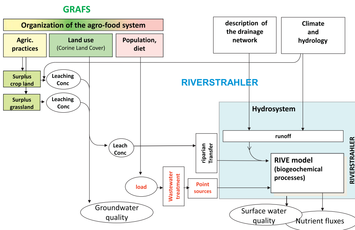
Fig. 2. Representation of the principles of the Grafs-Senèque-Riverstrahler modeling approach.
