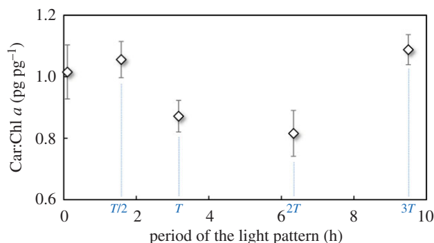
Figure 7. Car:Chl a ratio (pg pg -1 ) of Dunaliella salina as a function of T (no measurement could be carried out for T /3 due to the low biomass).
