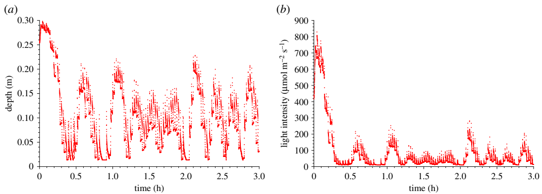
Figure 3. Depth (a) and light (b) pattern of the paragon trajectory.
