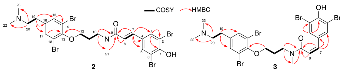
Figure 2. COSY and key HMBC correlations for psammaplysenes F ( 2 ) and G ( 3 ).
