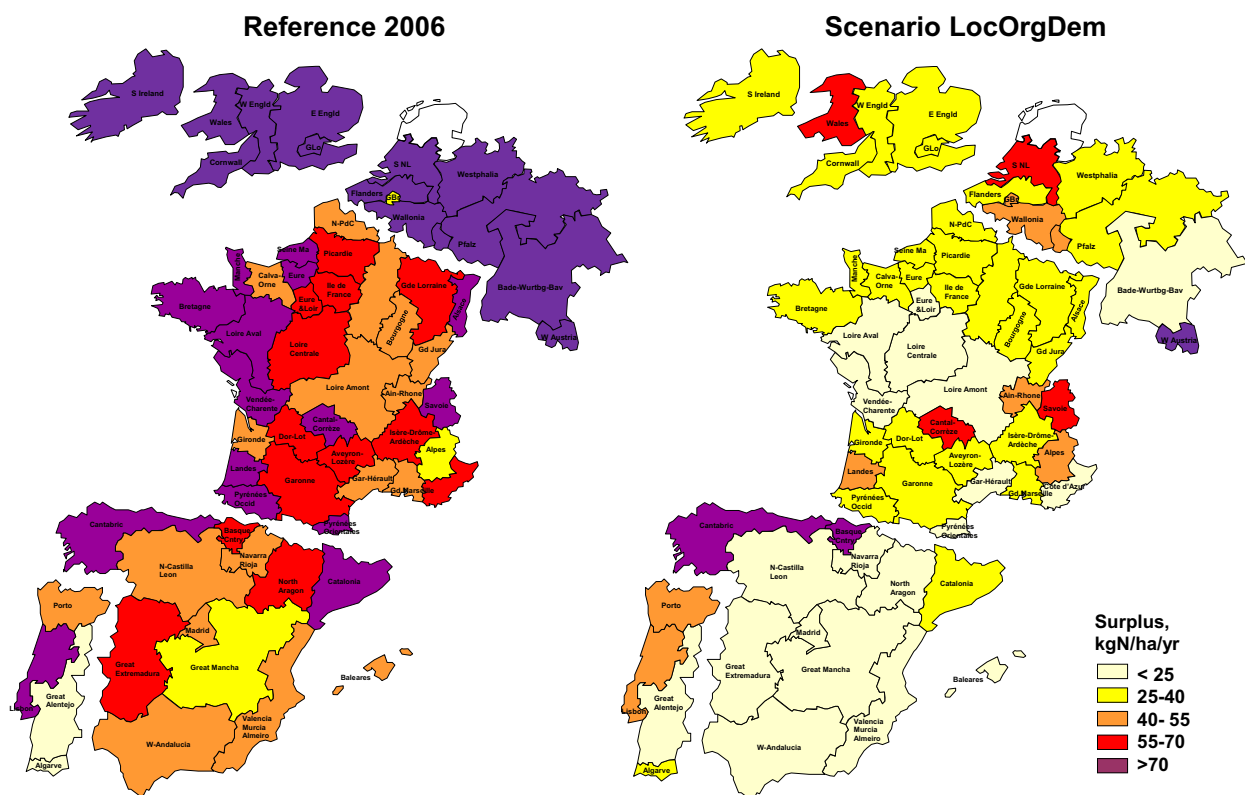
Fig. 4. Distribution of the average N soil balances on arable soils over the model domain in the Reference situation and in the LocOrgDem scenario.
