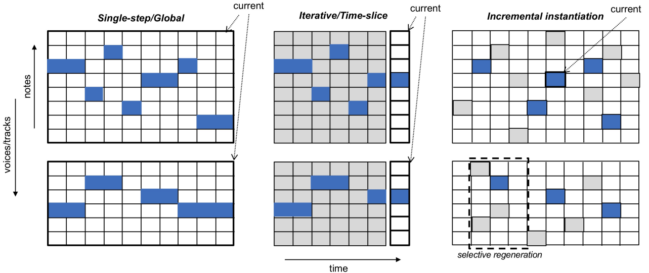
Figure 12: Strategies for instantiating notes during generation
