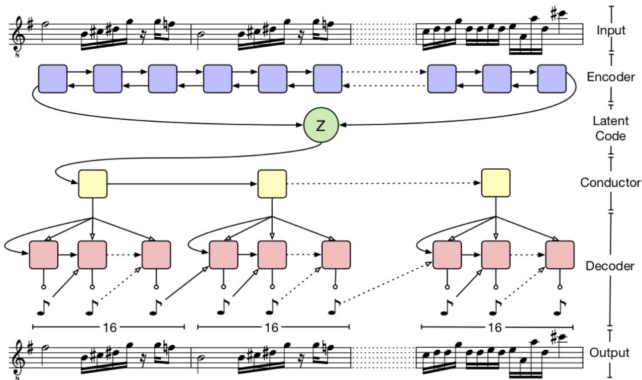
Figure 10: MusicVAE architecture. Reproduced from [RER + 18b] with permission of the authors
