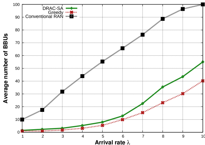
Fig. 12: Number of BBUs vs arrival rate \lambda
