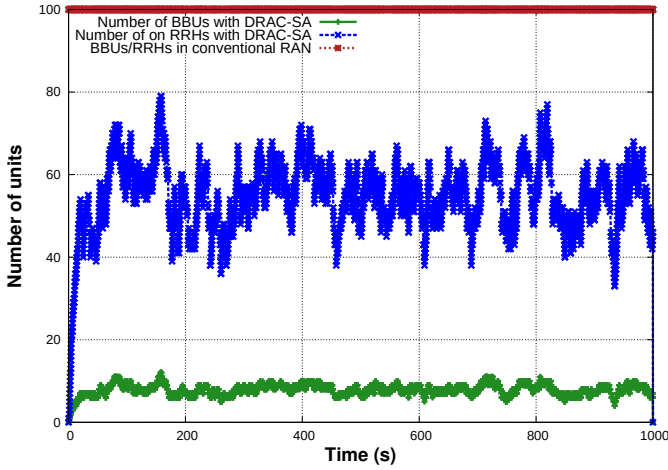
Fig. 9: Number of needed BBUs and on RRHs per time
