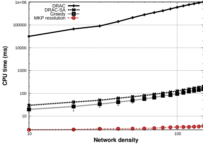
Fig. 4: CPU time vs number of UEs
