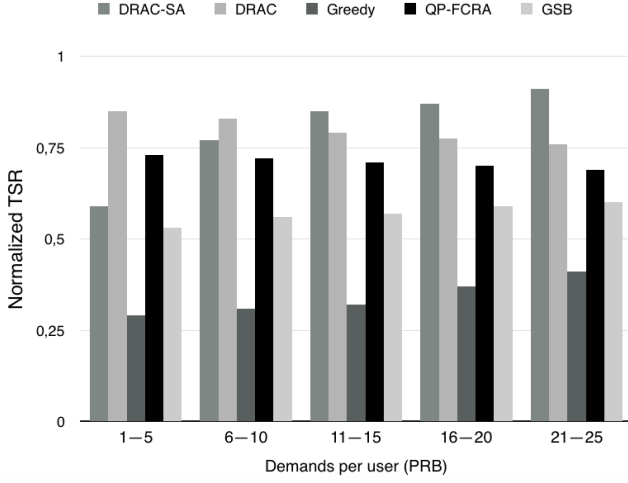
(a) SINR = 10 dB
