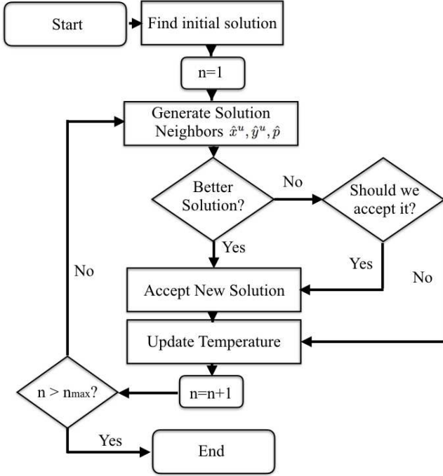
Fig. 2: DRAC-SA Flow Chart
