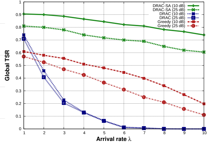
Fig. 10: Global TSR vs arrival rate \lambda
