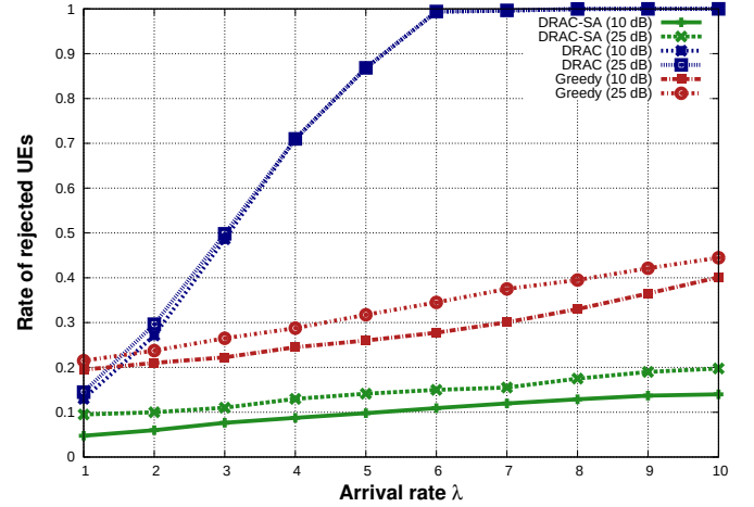
Fig. 11: Rejected users rate vs arrival rate \lambda
