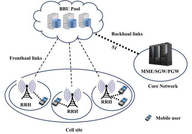
Fig. 1: Cloud Radio Access Network (C-RAN) Architecture
