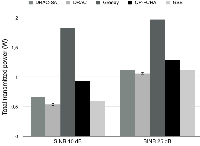
Fig. 8: Total RRHs transmitted power in C-RAN
