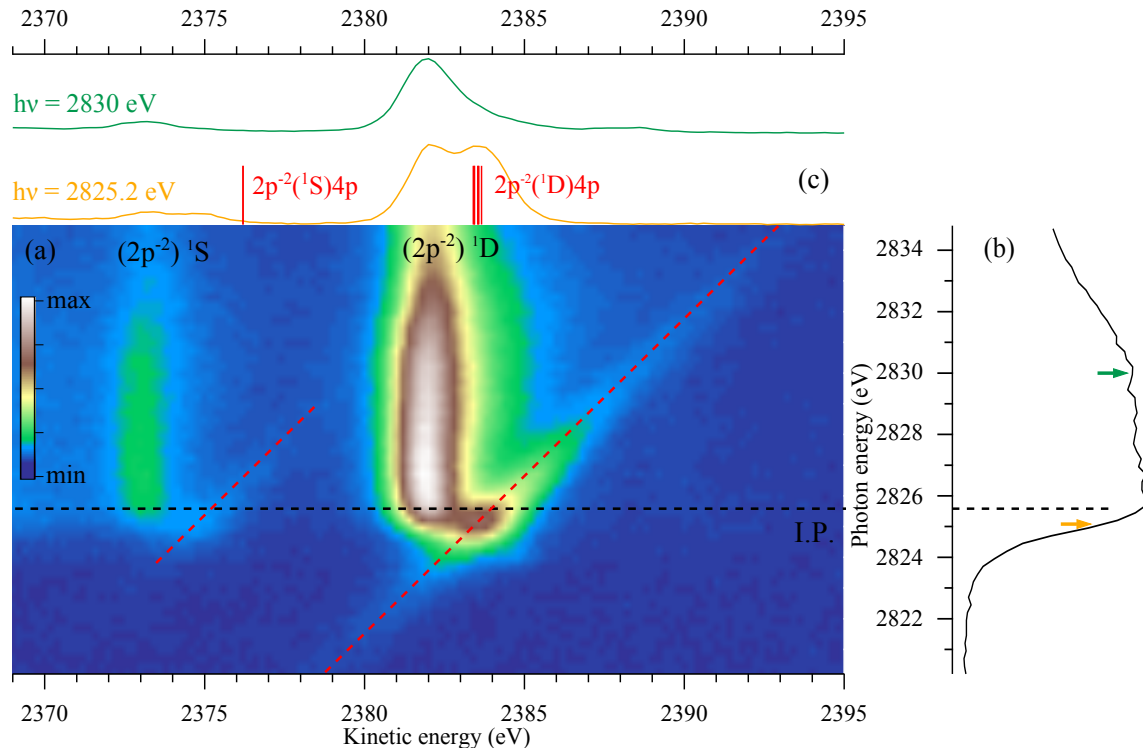
Figure 3: (a) 2D map showing the kinetic energy of the electrons emitted in KL_{2,3}L_{2,3} Auger decay vs the photon energy in the vicinity of the K-edge of aqueous Cl^- . (b) Experimental partial electron yield spectrum of Cl^- obtained after integrating over the kinetic energies of the Auger electrons. (c) Auger spectra at photon energies 2825.2 eV and 2830.0 eV. The vertical bars in the resonant Auger spectrum at 2825.2 eV indicate the the spectator Auger energies of the calculated doublet 2p^{-2}4p states of Cl^-(H_2O)_6 .
