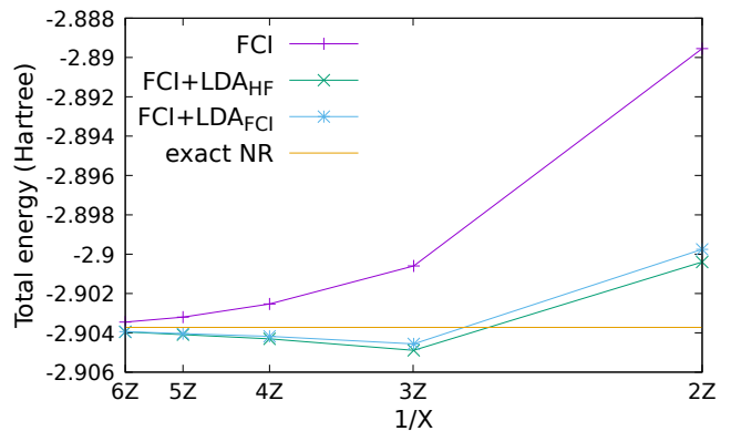
FIG. 4. Convergence of the total energy of the helium atom for FCI and FCI+LDA \Psi^{\mathcal{B}} , where \Psi^{\mathcal{B}} is either the HF or FCI wave function, as a function of the inverse of the cardinal number X of the AVXZ basis sets ( X = 2, 3, 4, 5, 6 ). The exact non-relativistic (NR) energy is also reported.
