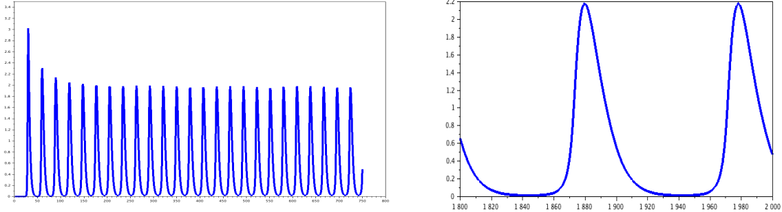
Figure 3: NUMERICAL SOLUTIONS OF THE EVOLUTION EQUATION (20) WITH DATA IN (34). ABSCISSAE ARE v . LEFT: FIRING RATE V_0(\mathcal{N}) = .75 + .15 \frac{\mathcal{N}}{1+\mathcal{N}} ; RIGHT: ZOOM ON TWO OSCILLATIONS.
