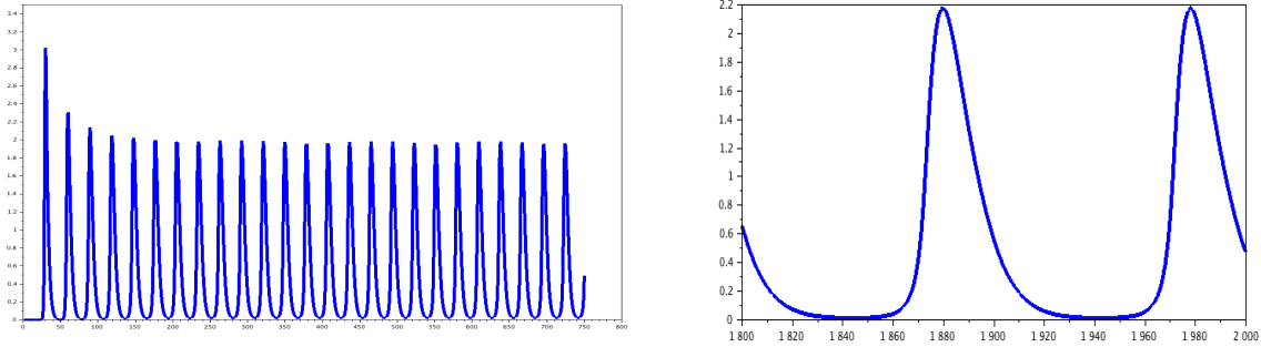
Figure 3: NUMERICAL SOLUTIONS OF THE EVOLUTION EQUATION (20) WITH DATA IN (34). ABSCISSAE ARE v . LEFT: FIRING RATE V_0(N) = .75 + .15 \frac{N}{1+N} ; RIGHT: ZOOM ON TWO OSCILLATIONS.
