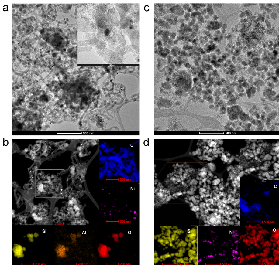
Fig. 13. Microscopic images of the catalysts after ESR reaction performed at 500 °C for 20 h; a) Ni 10 HAIBEA - TEM (Fig. 13a) and STEM (Fig. 13b); Ni 10 SiBEA - TEM (Fig. 13c) and STEM (Fig. 13d).
