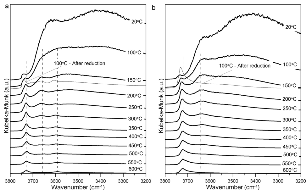
Fig. 7. DRIFTS spectra of Ni 10 HAIBEA (a) and Ni 10 SiBEA (b) catalysts recorded during thermal treatment in H 2 from 20 °C to 600 °C and subsequent cooling down to 100 °C.
