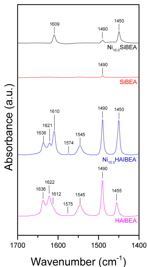
Fig. 9. FTIR spectra recorded at room temperature of HAIBEA, Ni 10 HAIBEA, SiBEA and Ni 10 SiBEA after adsorption of pyridine (133 Pa) for 1 h at room temperature and desorption at 150 °C.
