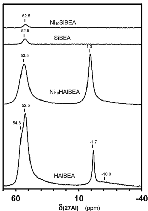
Fig. 5. ^{27}\text{Al} MAS NMR spectra of HAIBEAE, \text{Ni}_{10}\text{HAIBEAE} , SiBEAE and \text{Ni}_{10}\text{SiBEAE} .
