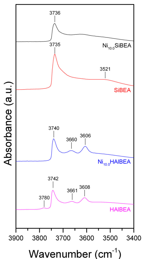
Fig. 8. FTIR spectra recorded at room temperature of HAIBEA, Ni 10 HAIBEA, SiBEA and Ni 10 SiBEA in the vibrational range of OH groups.
