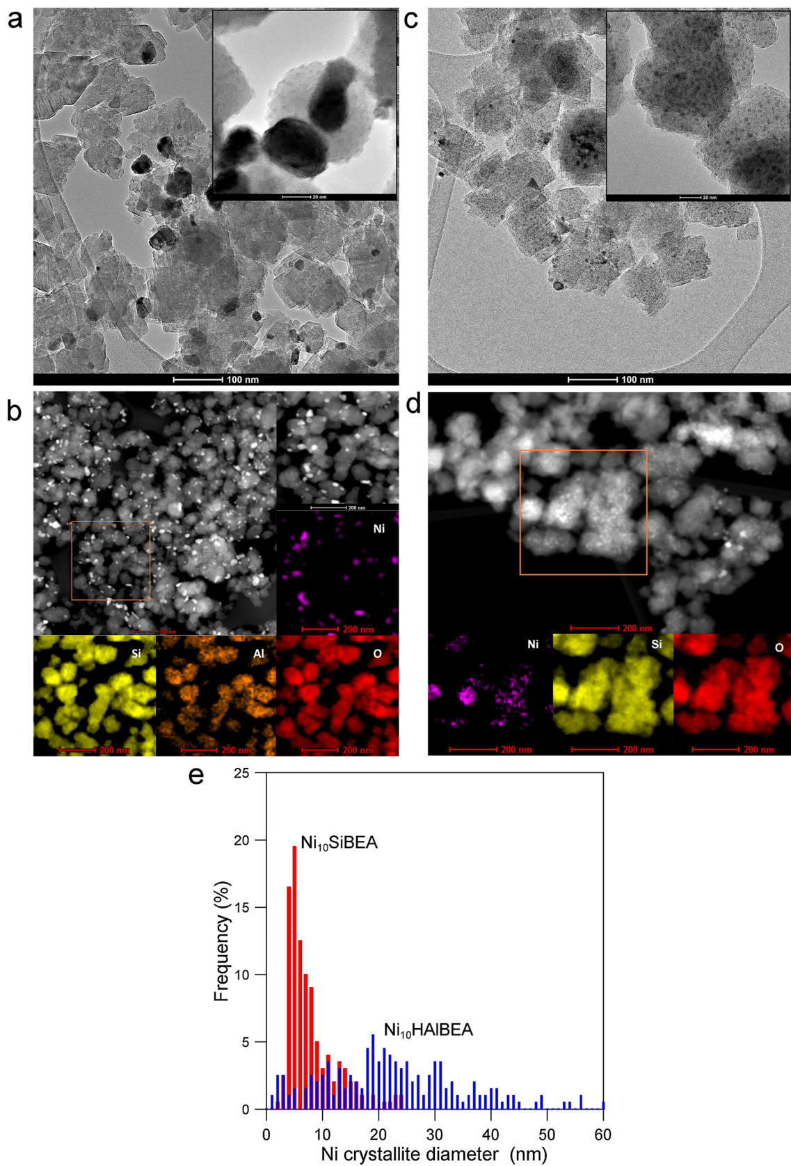
Fig. 2. a) TEM images of \text{Ni}_{10}\text{HAIBEA} catalyst after reduction, b) STEM images of \text{Ni}_{10}\text{HAIBEA} catalyst after reduction, c) TEM images of \text{Ni}_{10}\text{SiBEA} catalyst after reduction, d) STEM-EDS images of \text{Ni}_{10}\text{SiBEA} catalyst after reduction, e) nickel crystallite size distribution in catalysts.
