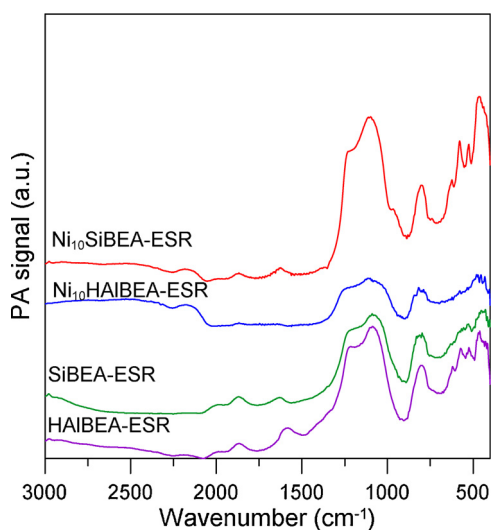
Fig. 14. FTIR/PAS studies of the zeolites and nickel catalysts after ESR reaction.
