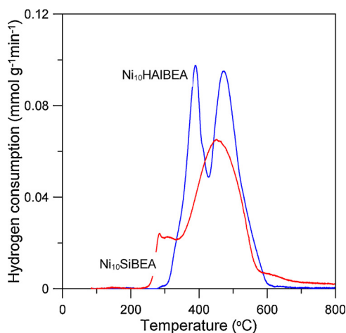
Fig. 10. Temperature-programmed reduction curves of nickel catalysts.
