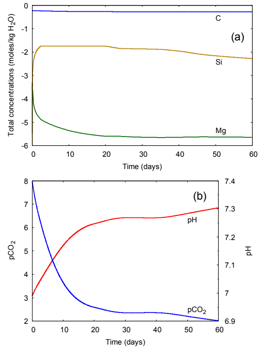
FIG. 4: a): time evolution of the concentration of elements in the aqueous solution (log scale); b): pH in the aqueous solution and \text{CO}_2 pressure p_{\text{CO}_2} from NANOKIN simulation.
