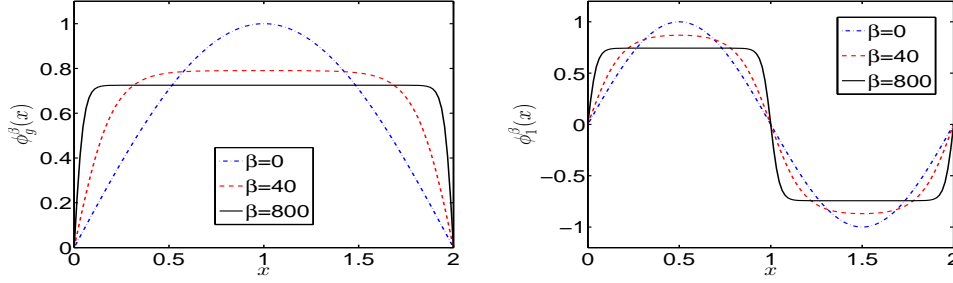
FIG. 2.1. Ground states \phi_g^\beta(x) (left) and first excited states \phi_1^\beta(x) (right) of GPE in 1D with \Omega = (0, 2) and a box potential for different \beta \geq 0 .
