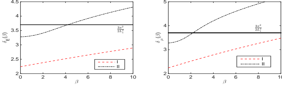
FIG. 2.5. Fundamental gaps in energy (left) and chemical potential (right) of GPE in 1D with \Omega = (0, 2) and non-convex trapping potentials: (I) V(x) = -10x^2 , and (II) V(x) = 10 \sin(10(x-1)) for different \beta \geq 0 .
