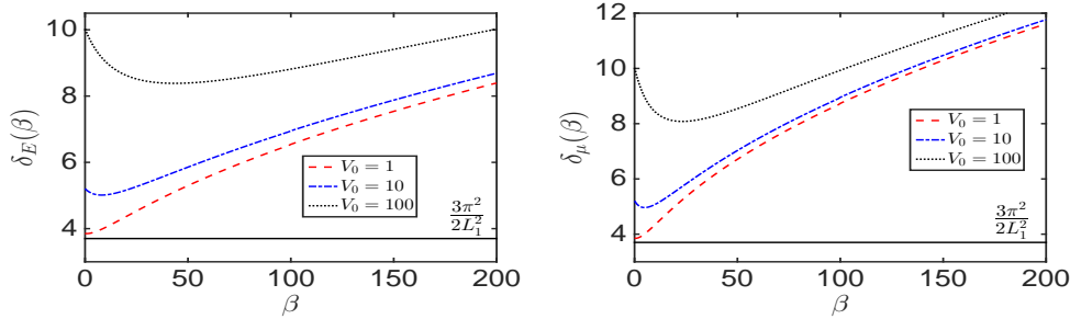
FIG. 2.4. Fundamental gaps in energy \delta_E(\beta) (left) and chemical potential \delta_\mu(\beta) (right) of GPE in 1D with \Omega = (0, 2) and V(x) = V_0(x - 1)^2 for different V_0 > 0 and \beta \geq 0 .
