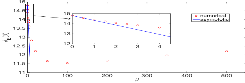
FIG. 2.8. The fundamental gaps in energy of GPE in 3D under a box potential with \Omega = (0, 1)^3 .
