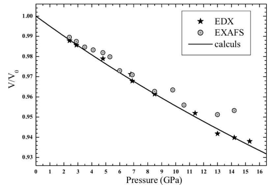
FIG. 10: Pressure dependence of the cell volume for the rock-salt phase upon decompression.
