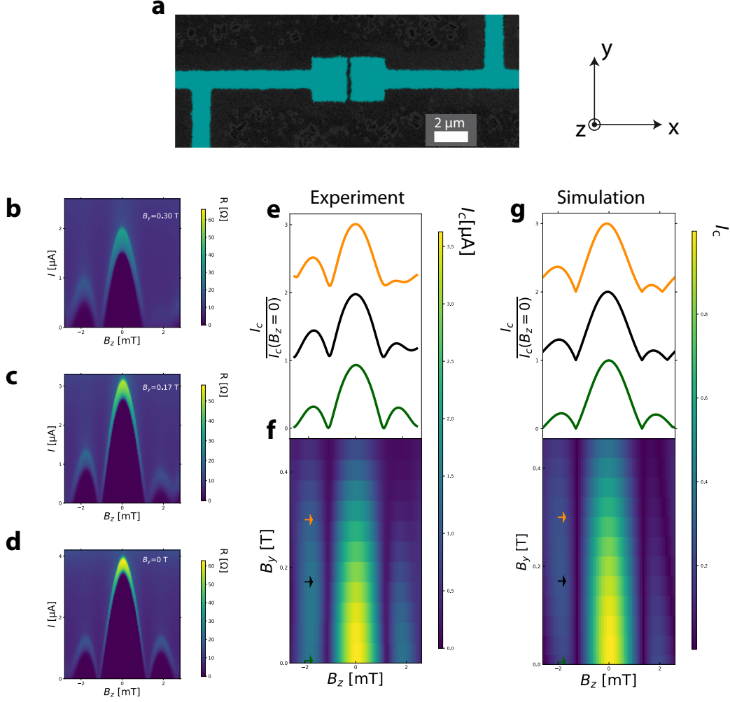
Figure 3: Asymmetric Fraunhofer pattern. a SEM image of a single junction device. The spacing between the two superconducting electrodes is L=150 nm and the width of the junction W=2 μm. bcd Resistance maps as function of current and perpendicular magnetic field B_z , for different values of the in-plane magnetic field B_y . The corresponding critical current curves are shown panel e. At zero in-plane magnetic field, panel d, the Fraunhofer pattern is symmetric with respect to B_z . The pattern becomes asymmetric upon increasing B_y . f Critical current map as a function of B_z and B_y showing the evolution from symmetric Fraunhofer pattern at B_y = 0 to the asymmetric Fraunhofer pattern for B_y > 0 . g Numerical simulation of the anomalous Fraunhofer pattern due to disorder and spin-orbit coupling. The model is described in the Supp. Note 4.
