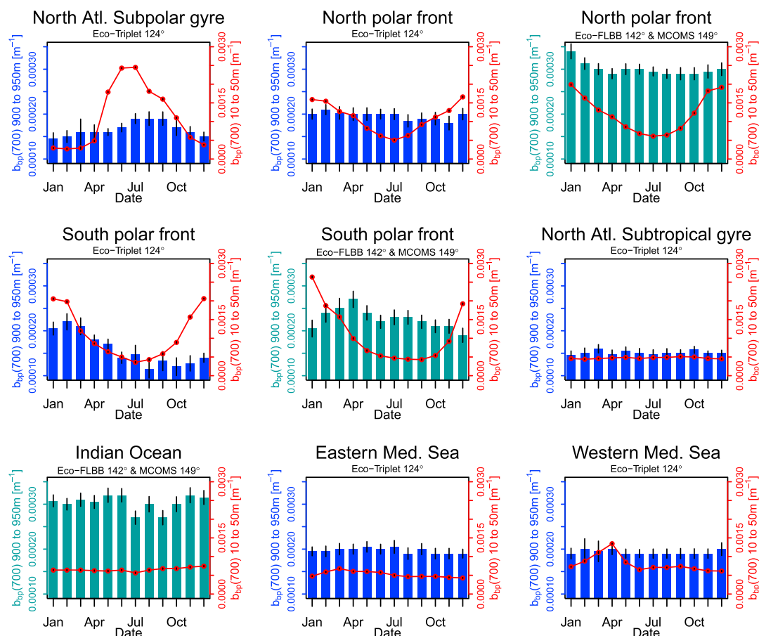
Figure 3. Histograms of monthly b_{bp}(700) median values and resulting annual cycle at different oceanic regions with at least 10 profiles from three distinct floats per month, with blue denoting data with Eco-triplets and green combined Eco-FLBB and MCOMS at both surface (10–50 m, red lines) and 900–950 m. Black lines represent the spread of the median.
